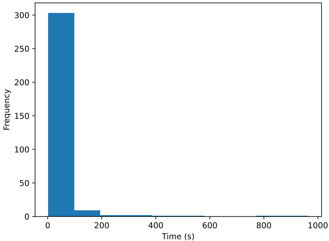
BFS time distribution
