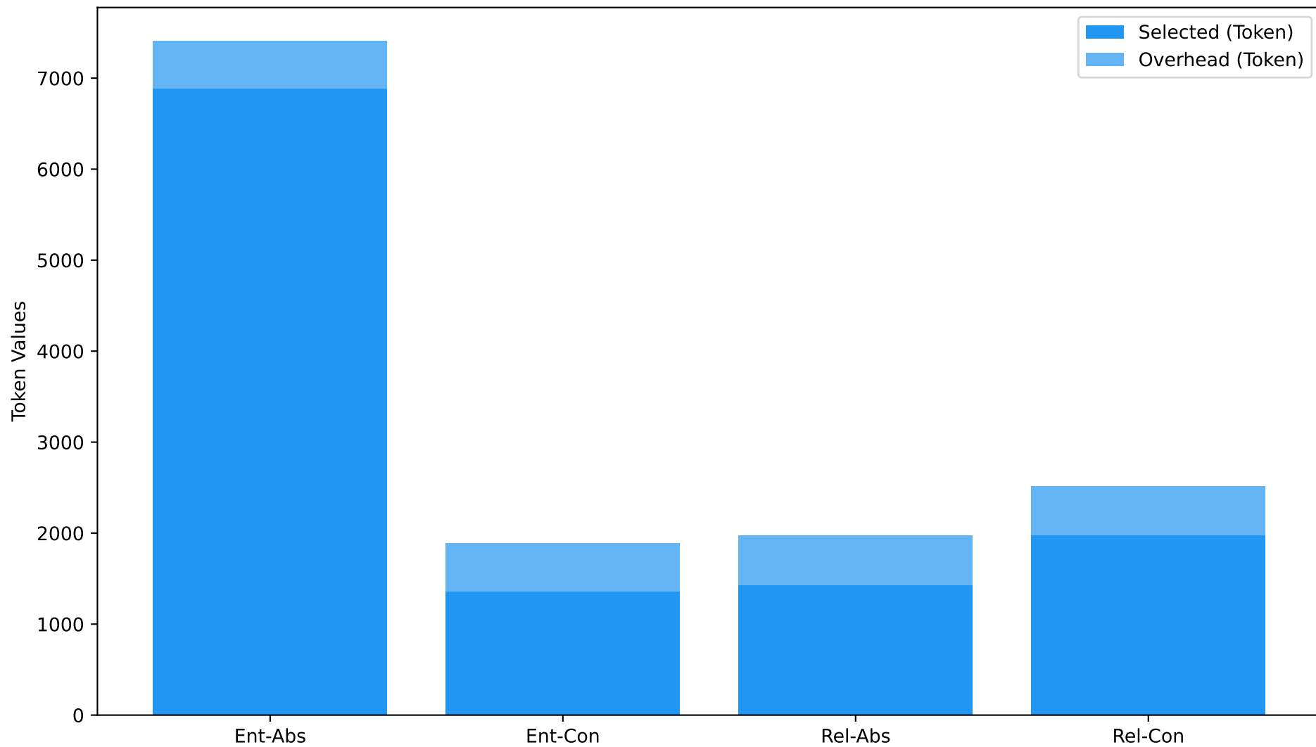
Stacked Bar Chart for Token (Selected and Overhead)
