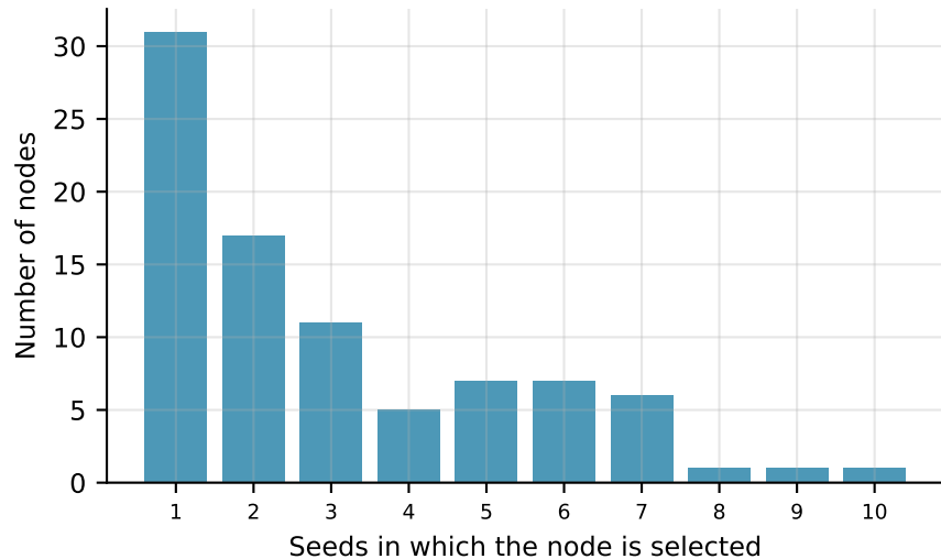
LINK: broker selection stability ensemble=30, vote=23, overlap=22
