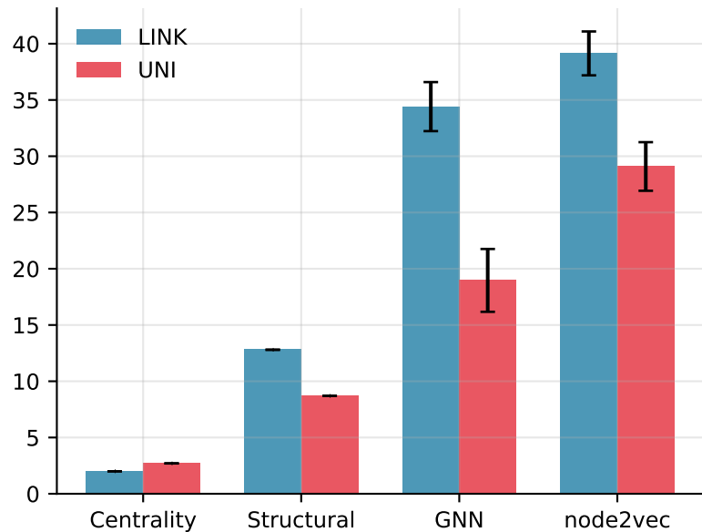
Neighbourhood enrichment
