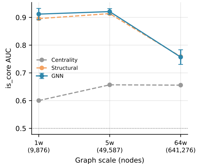
AUC: GNN advantage vanishes with scale
