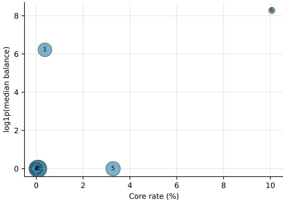
LINK: wealth vs structural power (fused, \rho=+0.20 )
