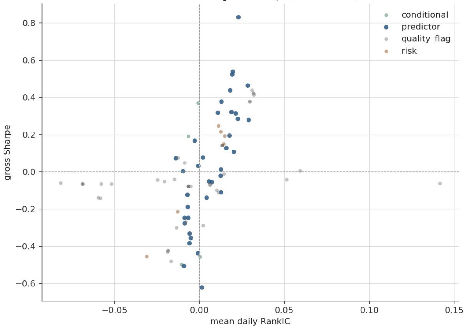
OOS RankIC vs gross Sharpe (all 92 fields)
