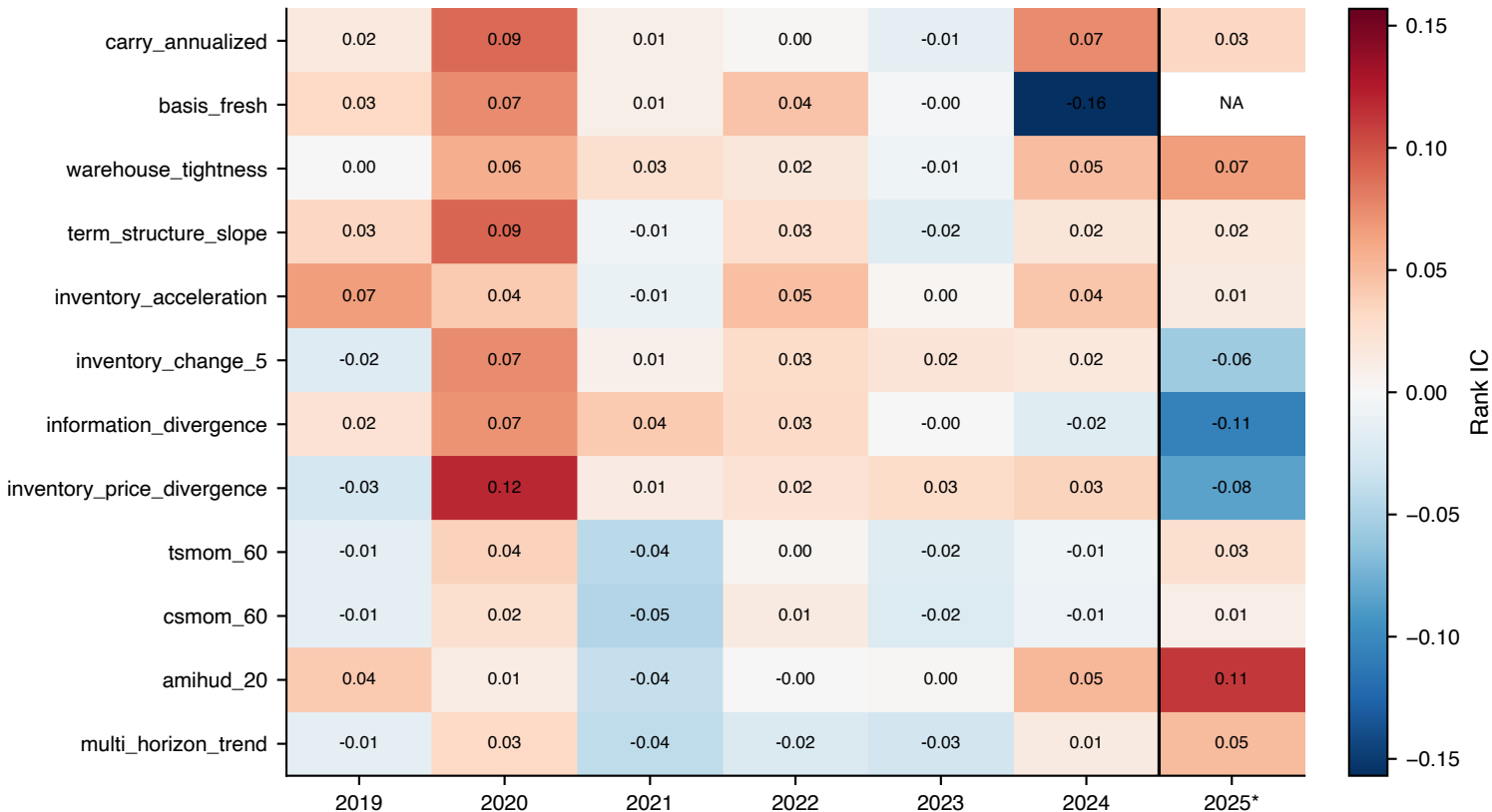
Yearly Rank IC stability (2019–2024) + sealed 2025
