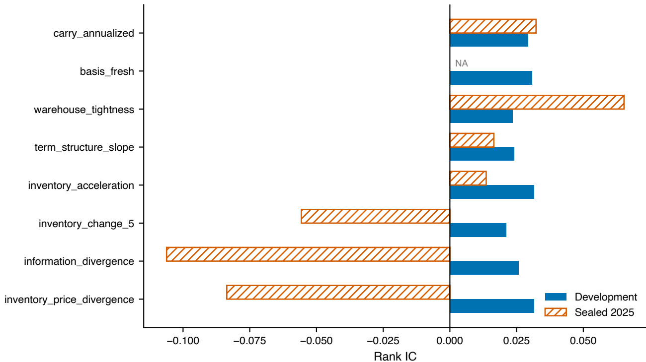
B-class candidates: development vs. sealed 2025
