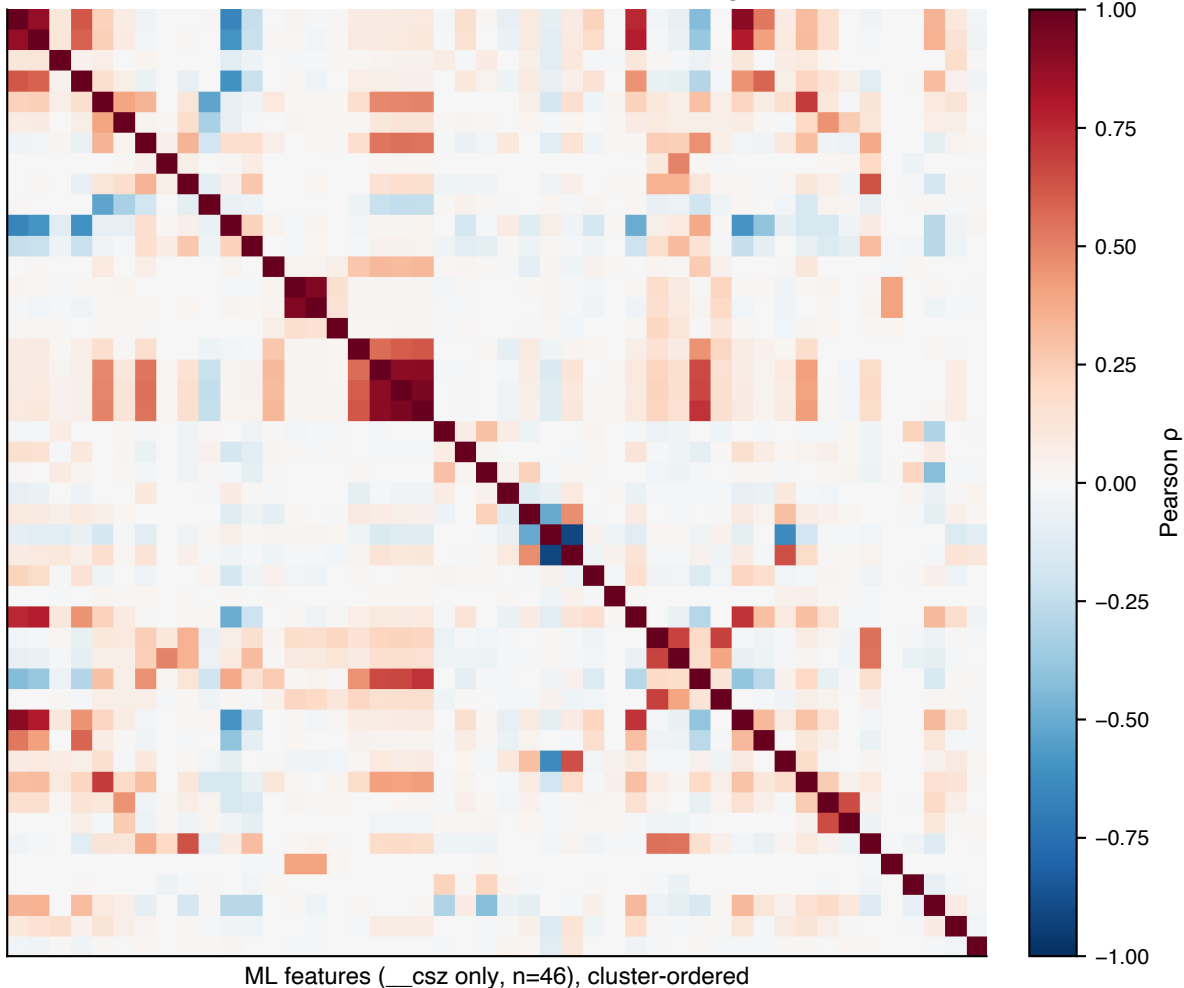
Feature correlation matrix (redundancy diagnosis)
