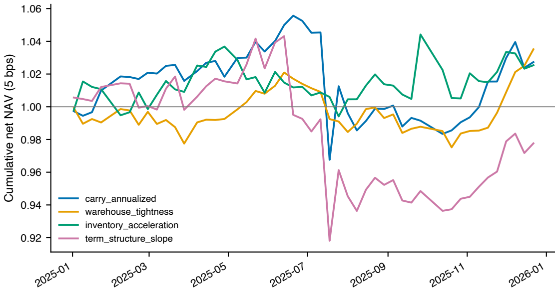
Sealed 2025 long-short paths (sign-persistent B candidates)
