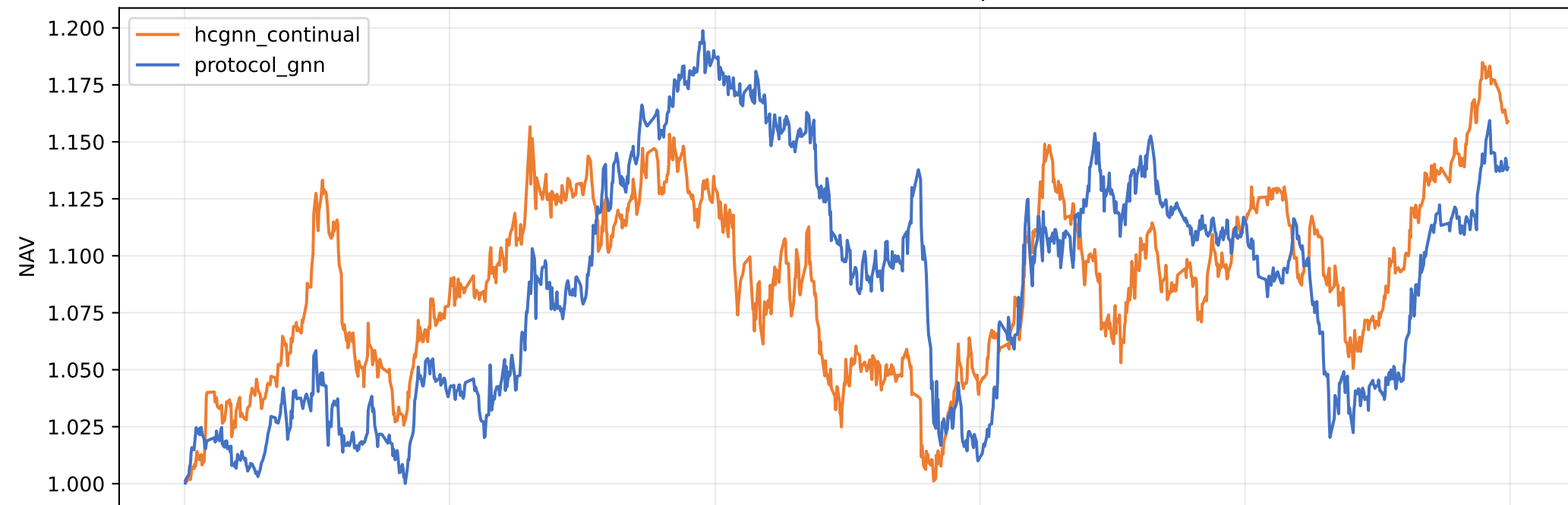
OOS net asset value (5 bps)
