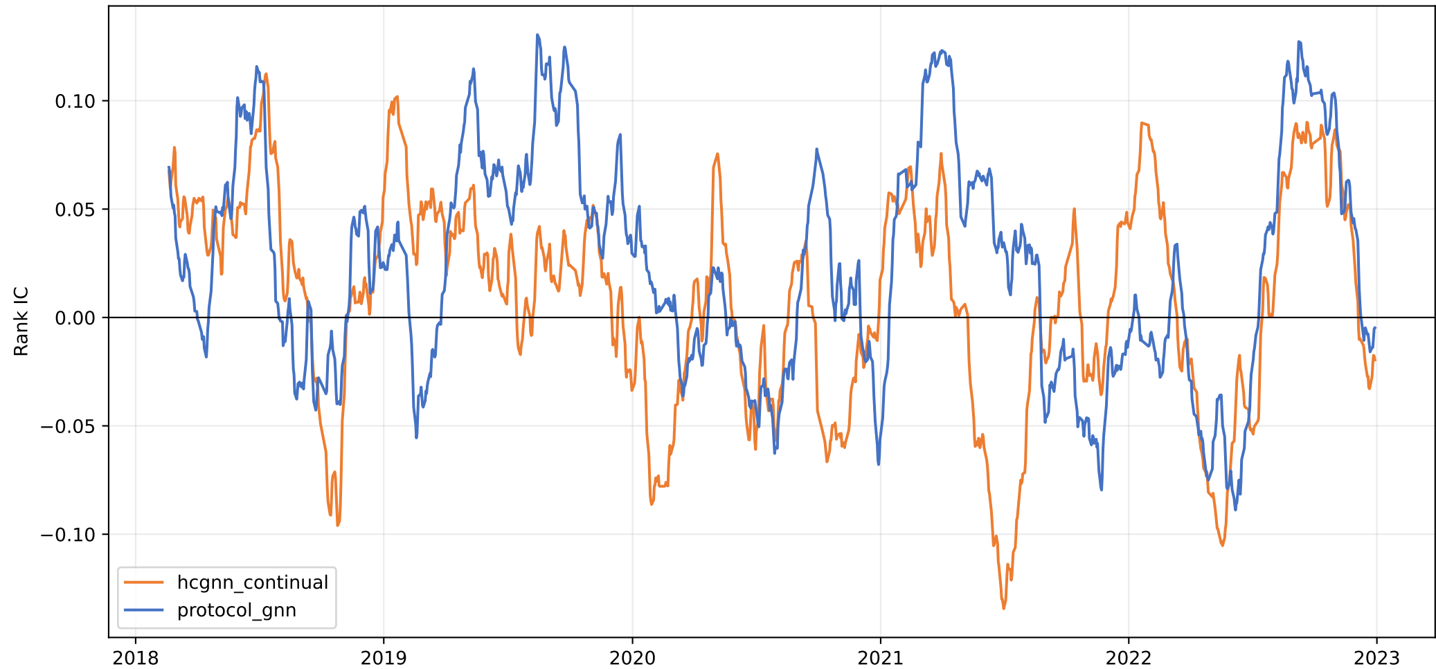
60-day rolling Rank IC
