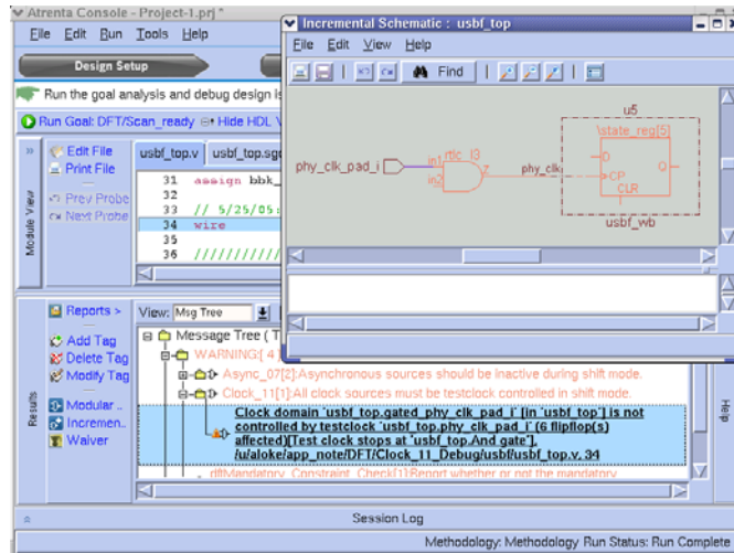
FIGURE 27. Clock_11 violations
