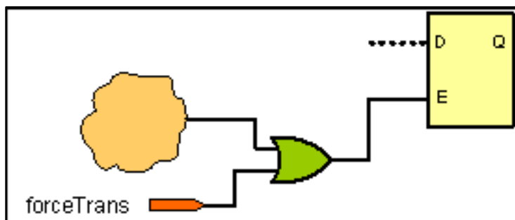
FIGURE 13. DFT Logic to Force Latch Transparency
