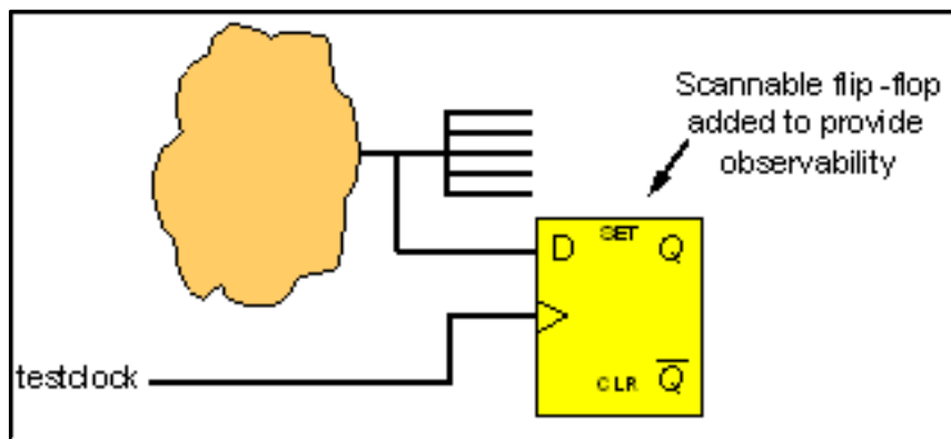
FIGURE 15. Observation Testpoint
