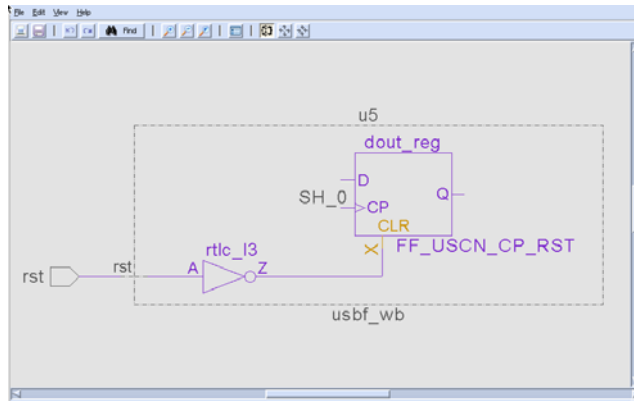
FIGURE 29. Async_07 violations
