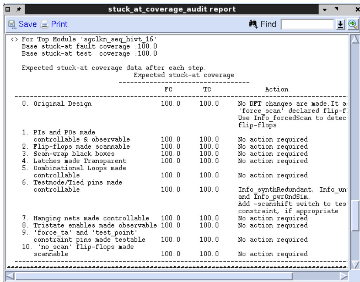
FIGURE 33. Example of the stuck_at_coverage_audit report
