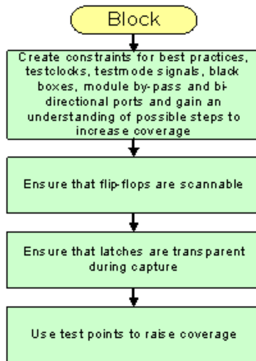
FIGURE 5. Block-level Flow
