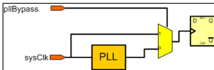
FIGURE 11. PLL bypass
