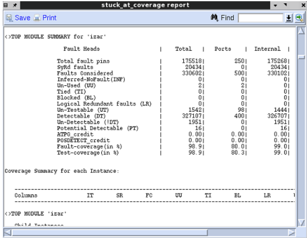
FIGURE 31. Fault status
