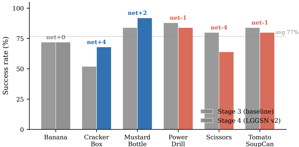
Per-object grasp success rate: Stage 3 vs Stage 4 ( N = 25 seeds)
