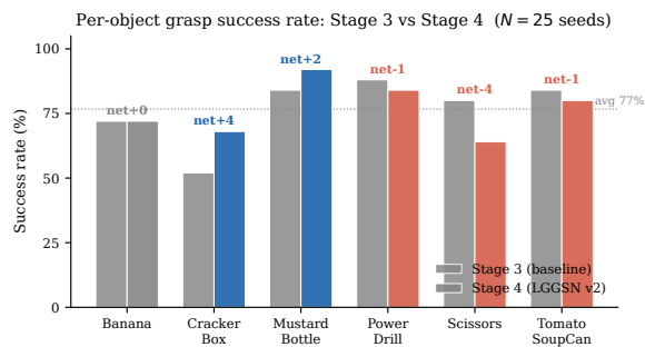
Figure 1. Per-object grasp success rate for Stage 3 (grey) and Stage 4 (blue = positive net, red = negative net). Annotations show the net change per object. The overall rate is 76.7 % in both conditions ( N = 25 seeds).
