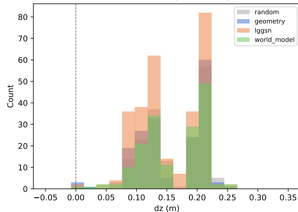
dz Distribution (Successes)
