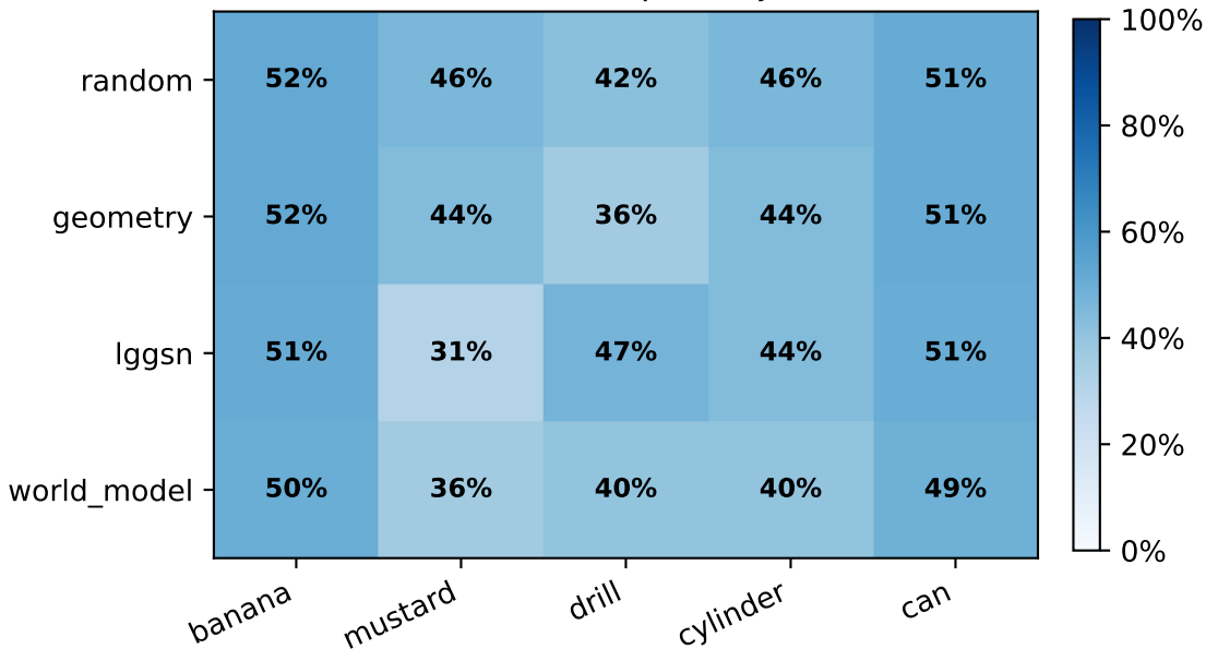
Bilateral Contact Rate per Object × Method
