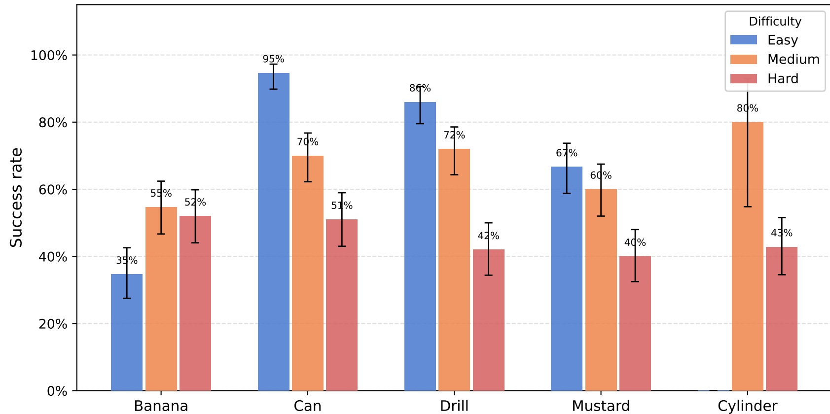
Grasp Success Rate vs. Difficulty — 50 seeds × 5 objects (bars averaged across geometry + random methods; 95% Wilson CI)
