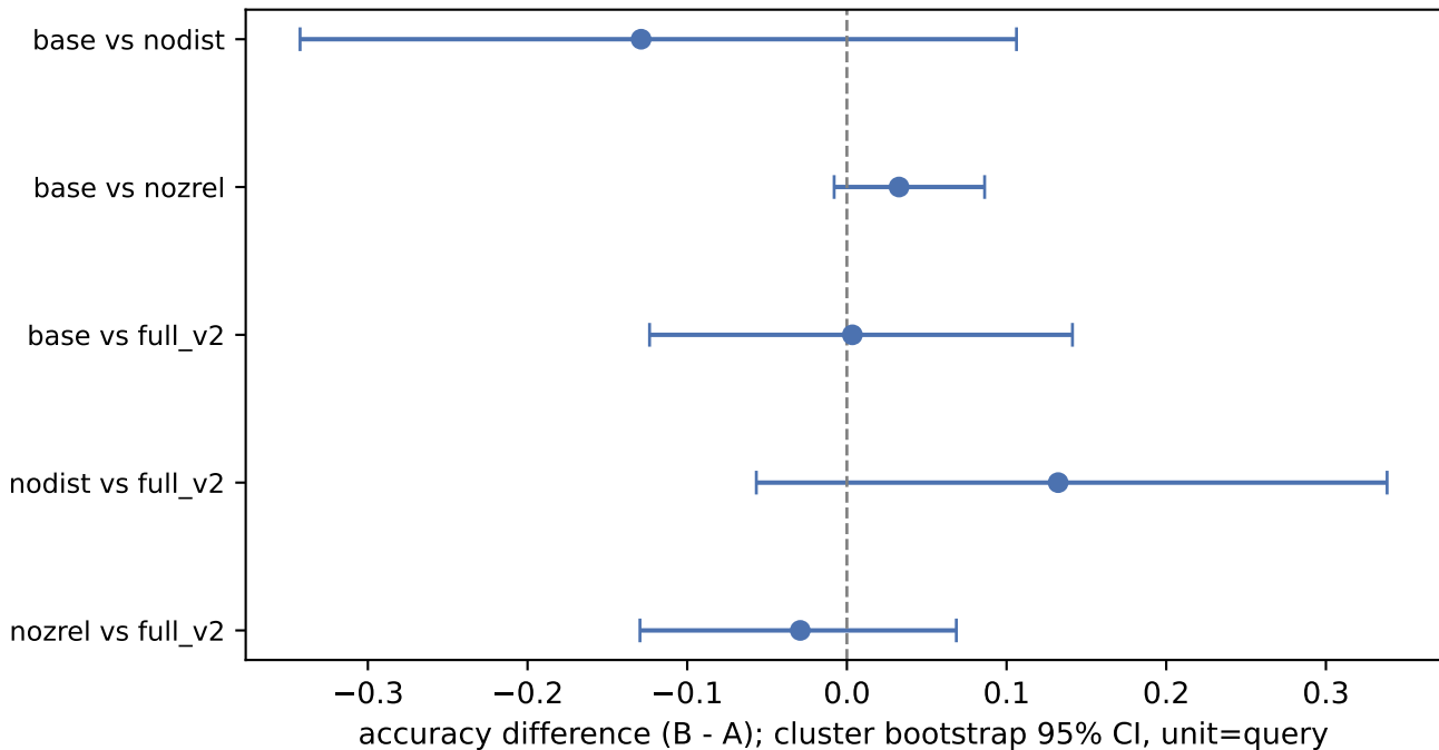
LGGSN core-matrix accuracy difference with 95% CI
