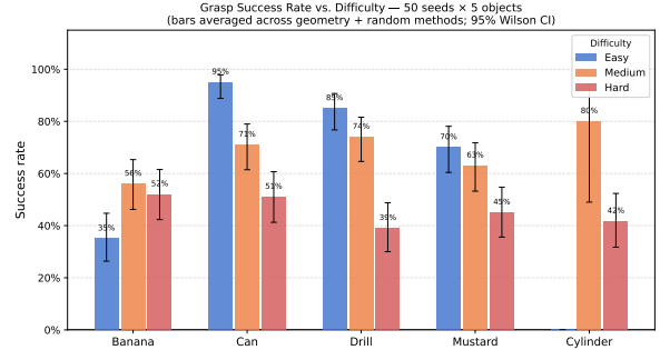
Figure 4. Grasp success rate on SO-ARM101 (MuJoCo) across three difficulty levels (50 seeds \times 5 objects; bars averaged over geometry and random methods; 95 % Wilson CI). Can and Drill degrade monotonically; Banana inverts because a centred top-down approach always contacts the curved tip in easy mode.
