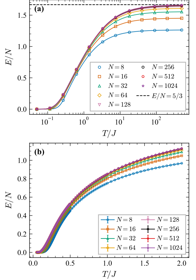
FIG. 3. Energy per queen E/N vs. temperature for N = 8 to 1024. (a) Logarithmic temperature scale over the full range T = 0.05 – 400 J ; the dashed line marks the analytical N \rightarrow \infty high- T limit E/N = 5/3 . (b) Linear scale, zoomed to T \leq 2 J , with error bars.
