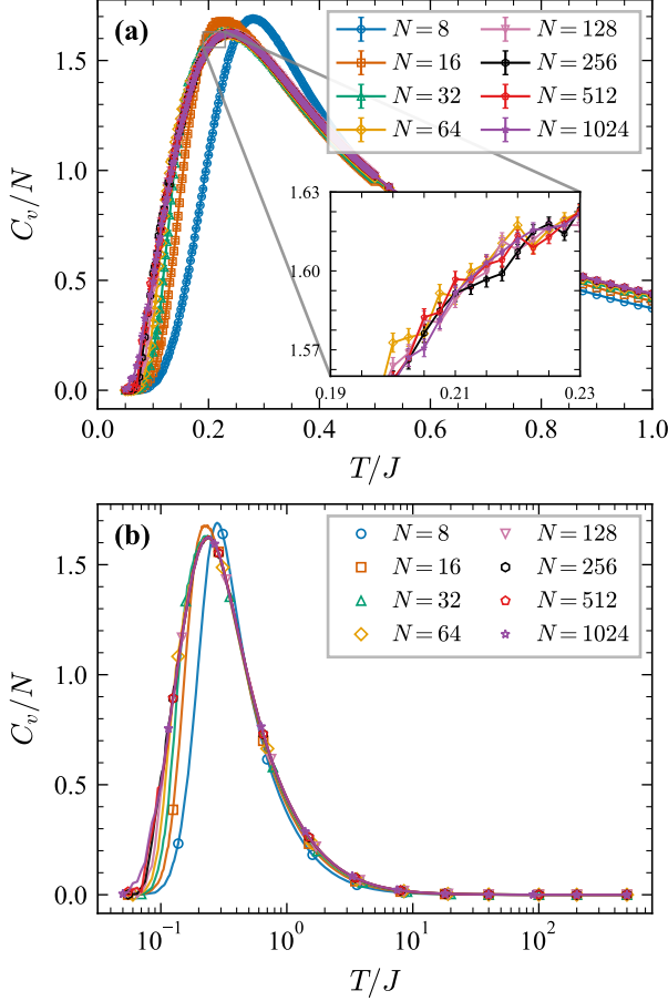
FIG. 4. Specific heat per queen C_v/N vs. T for N = 8 to 1024. (a) Peak region ( T \leq 1 J , linear scale) with error bars; the inset enlarges the peak vicinity ( T = 0.19 – 0.23 J ) for N \geq 64 , revealing subtle size-dependent shifts in the peak height and position. (b) Full temperature range on a logarithmic T scale. The curves for N \geq 32 collapse onto a single function, confirming convergence to the thermodynamic limit.
