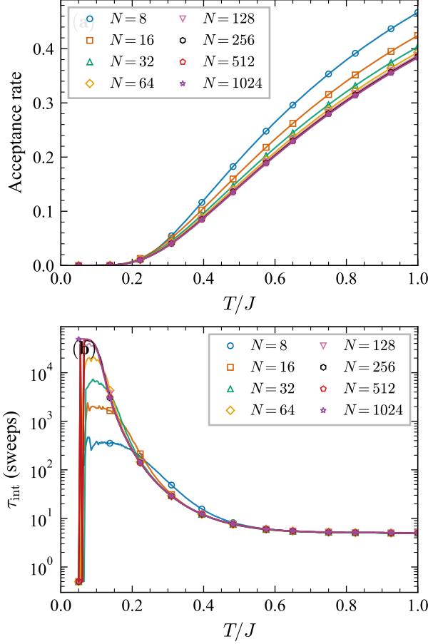
FIG. 2. Convergence diagnostics for the Monte Carlo simulations. (a) Acceptance rate of the Kawasaki (queen–vacancy exchange) moves as a function of temperature for N = 8 to 1024. The rate drops below 10^{-5} for T \lesssim 0.1 J and rises monotonically, reaching 0.38–0.47 at T = 1 J . (b) Integrated autocorrelation time \tau_{\text{int}} of the energy in units of sweeps (log scale). The sharp peak at T \approx 0.055 – 0.10 J reflects low-temperature freezing and lies well below the specific heat maximum T^* \approx 0.235 J ; at T^* itself, \tau_{\text{int}} \approx 85 – 200 sweeps, yielding more than 5 \times 10^5 independent samples from 10^8 sweeps.
