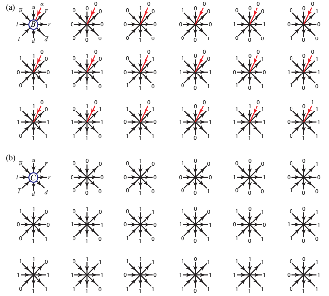
FIG. 5. The 17 nonzero elements of the site tensor B [Eq. (16)]. Each diagram shows a lattice site with eight bond indices carrying binary attack signals (0: absent, 1: present); red arrows mark active signals. The first 16 elements correspond to empty sites ( p = 0 ) with all 2^4 combinations of independent pass-through signals along the four constraint channels (column, row, and two diagonal families). The 17th element (bottom right) represents an occupied site ( p = 1 ): all incoming signals are 0 and all outgoing signals are 1.
