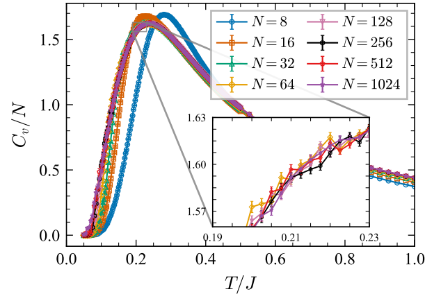
FIG. 4. Specific heat per queen C_v/N vs. T for N = 8 –1024 in the peak region ( T \leq 1 J , linear scale) with error bars. Inset: zoom into the peak for N \geq 32 . The curves for N \geq 32 collapse onto a single function, confirming convergence to the thermodynamic limit.
