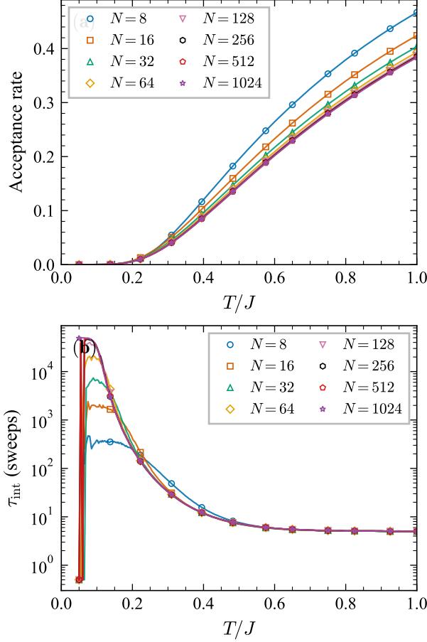
FIG. 2. Convergence diagnostics for the Monte Carlo simulations. (a) Acceptance rate of the Kawasaki (queen–vacancy exchange) [LW:consider making this log y scale] moves as a function of temperature for N = 8 –1024. The rate drops below 10^{-5} for T \lesssim 0.1 J and rises monotonically, reaching 0.38–0.47 at T = 1 J . (b) Integrated autocorrelation time \tau_{\text{int}} of the energy in units of sweeps (log scale). The sharp peak at T \approx 0.055 – 0.10 J reflects low-temperature freezing and lies well below the specific heat maximum T^* \approx 0.235 J ; at T^* itself, \tau_{\text{int}} \approx 85 –200 sweeps, yielding more than 5 \times 10^5 independent samples from 10^8 sweeps. [LW:legend (b) overlapped with curve]
