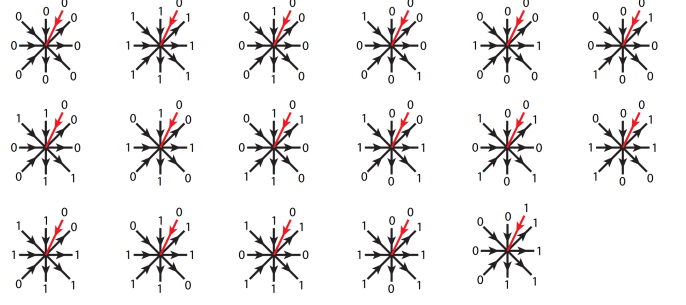
FIG. 5. The 17 nonzero elements of the site tensor T [Eq. (14)]. Each diagram shows a lattice site with eight bond indices carrying binary attack signals (0: absent, 1: present); red arrows mark active signals. The first 16 elements correspond to empty sites ( p = 0 ) with all 2^4 combinations of independent pass-through signals along the four constraint channels (column, row, and two diagonal families). The 17th element (bottom right) represents an occupied site ( p = 1 ): all incoming signals are 0 and all outgoing signals are 1.
