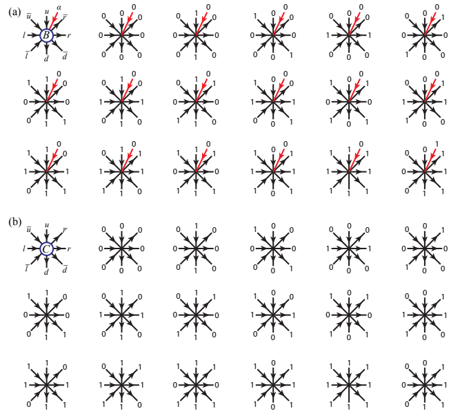
FIG. 5. The 17 nonzero elements of the site tensor \mathcal{T} [Eq. (16)]. Each diagram shows a lattice site with eight bond indices carrying binary attack signals (0: absent, 1: present); red arrows mark active signals. The first 16 elements correspond to empty sites ( p = 0 ) with all 2^4 combinations of independent pass-through signals along the four constraint channels (column, row, and two diagonal families). The 17th element (bottom right) represents an occupied site ( p = 1 ): all incoming signals are 0 and all outgoing signals are 1.
