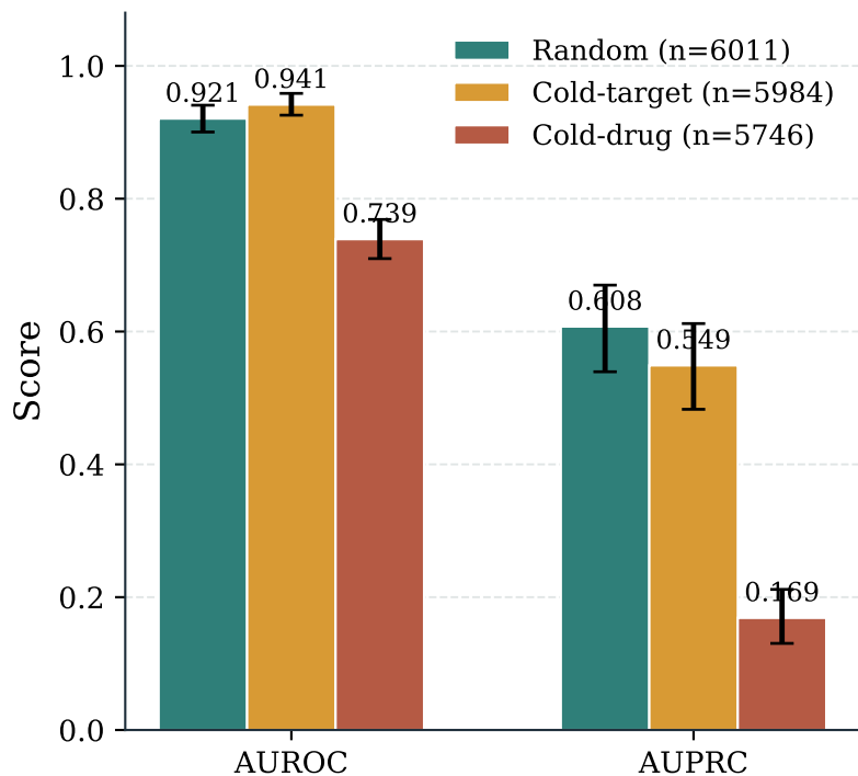
A Ranking metrics with 95% bootstrap CI
