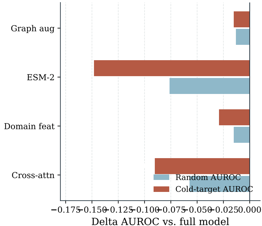
B Performance drop after removing each component
