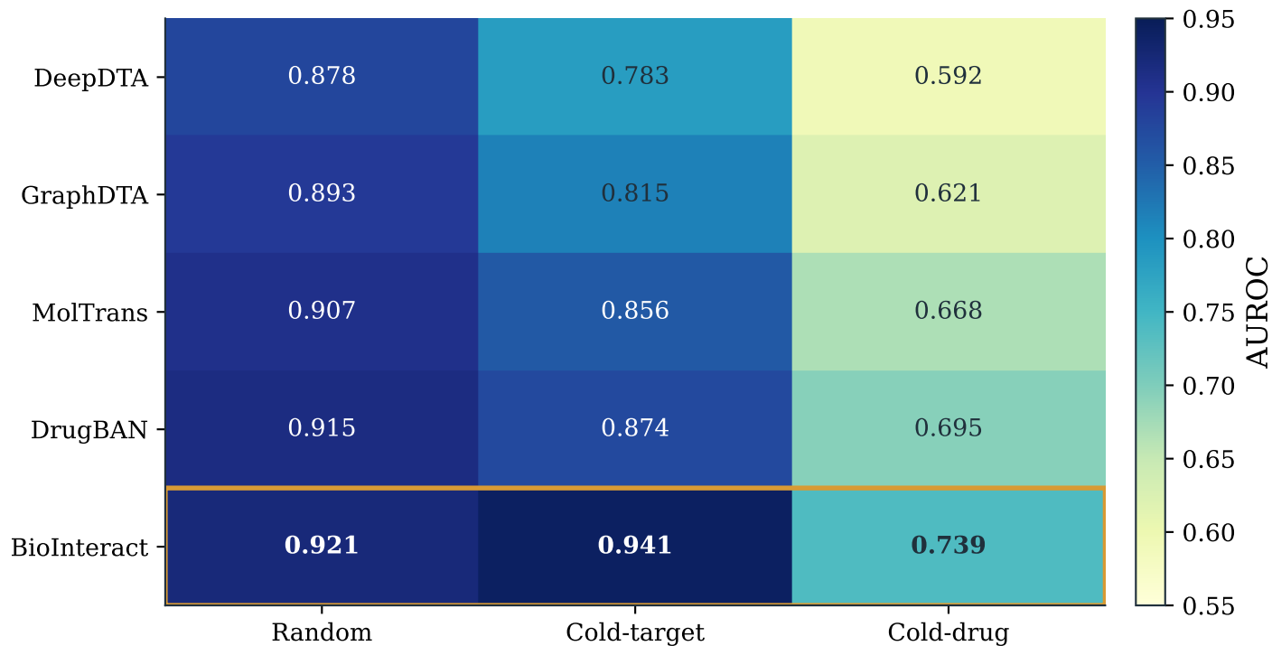
AUROC across data splitting protocols
