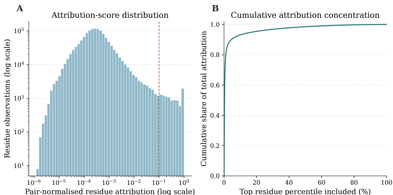
Figure 4. Attention sparsity analysis. (A) Histogram of the archived pair-normalised per-residue attention scores across all 1,506 positive Davis pairs (1,301,380 observations; logarithmic axes); the dashed line denotes the 0.1 sparsity threshold. (B) Cumulative attribution mass after sorting those same scores in descending order. The 99.2 % value is an attribution-concentration statistic, not a claim about a contiguous protein-surface region.
