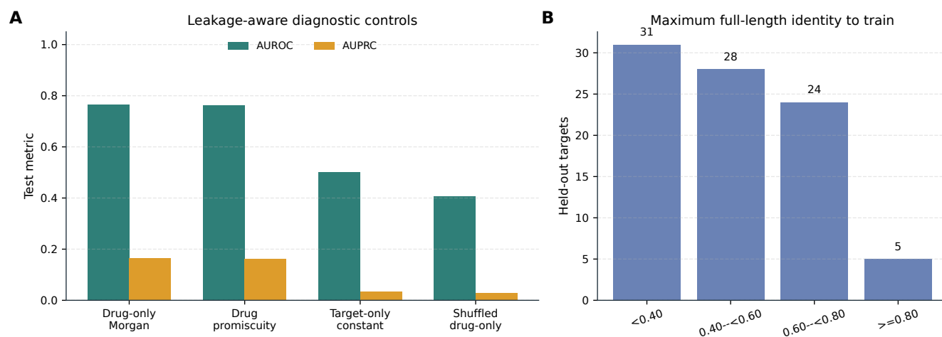
Figure 2. Diagnostic controls and target-relatedness audit. Panel A: leakage-aware controls on the exact-sequence-grouped cold-target test. Drug-only and drug-promiscuity scores use no target representation; the target-only constant is the only target-only control that does not use held-out target labels. Panel B: number of held-out targets by maximum full-length global sequence identity to any training target.
