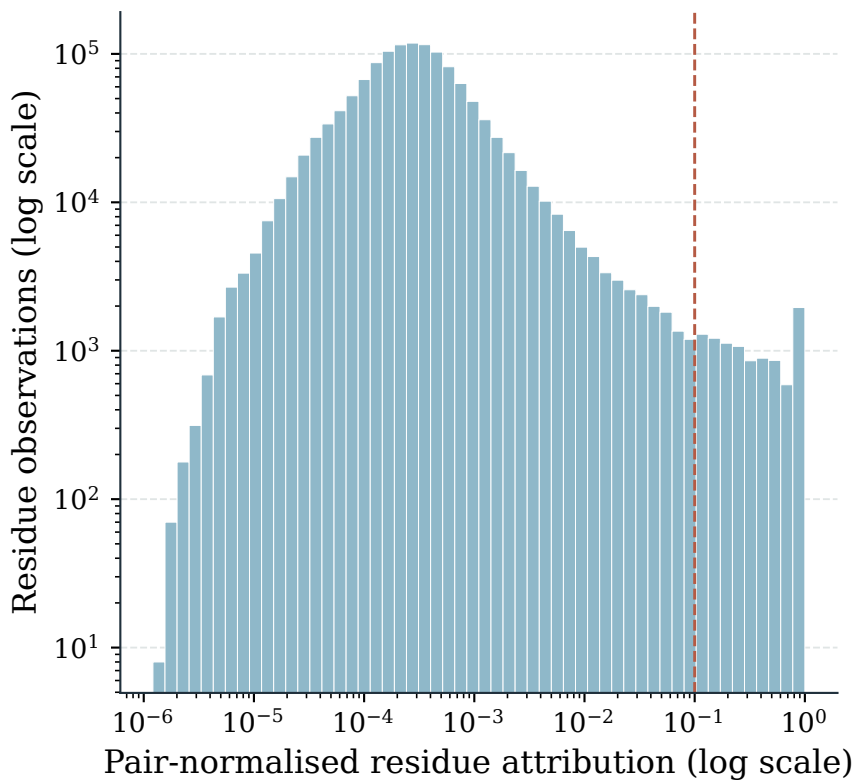
Attribution-score distribution
