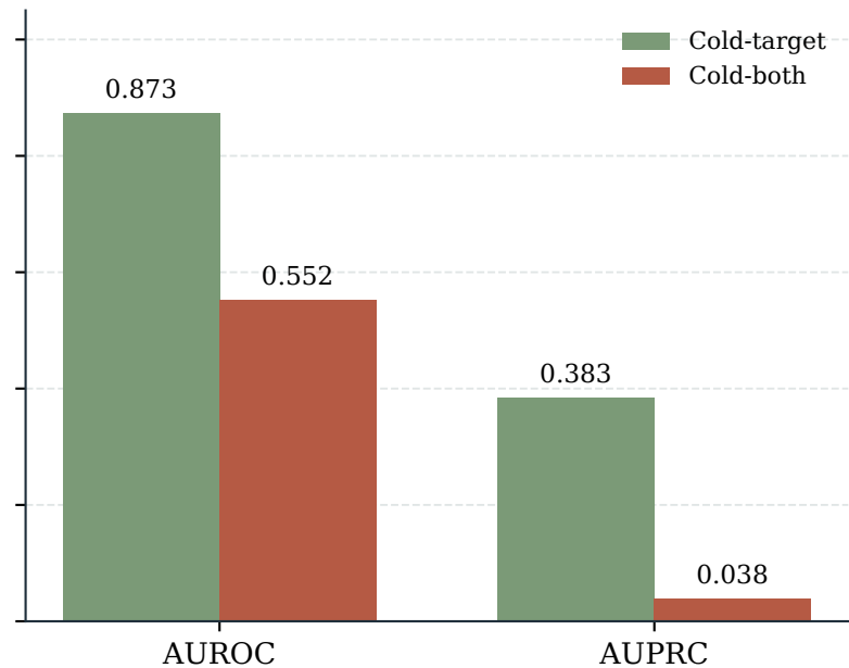
B Exact-sequence-grouped within-Davis tests
