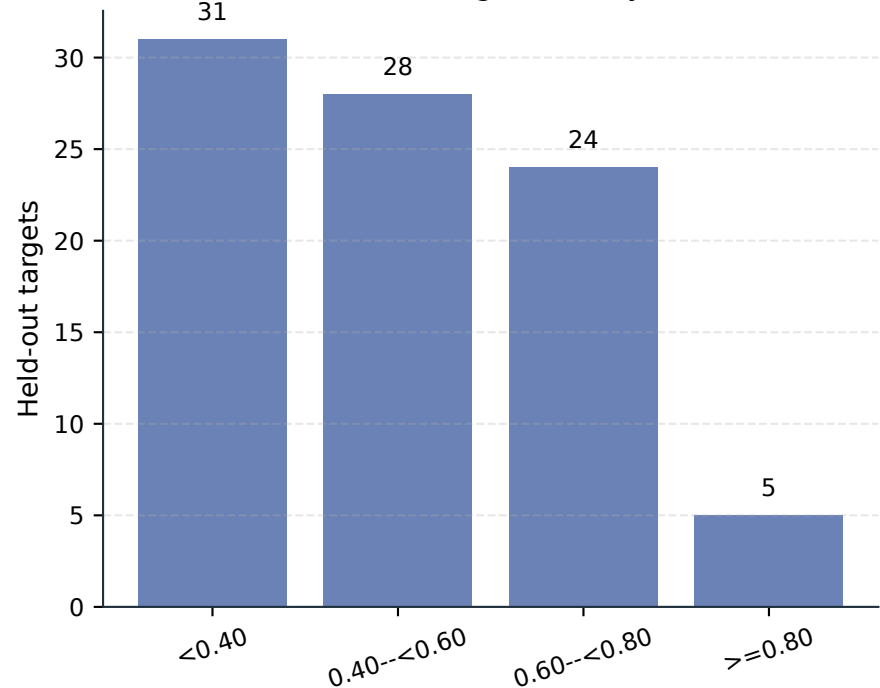
Maximum full-length identity to train
