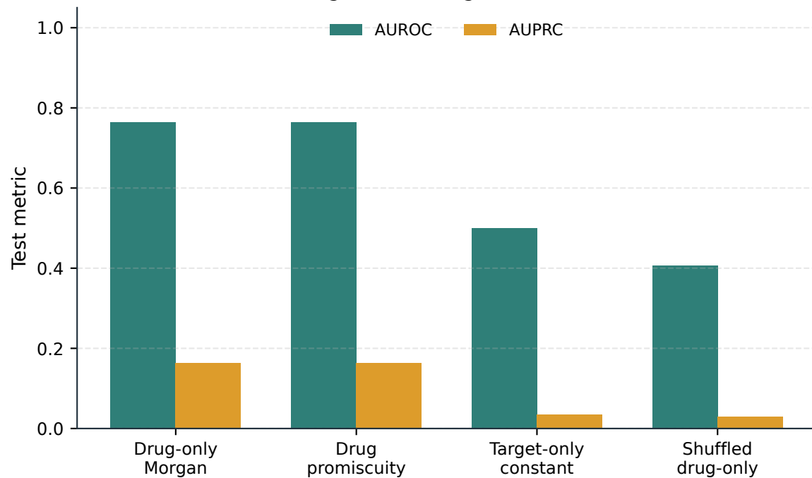
Leakage-aware diagnostic controls
