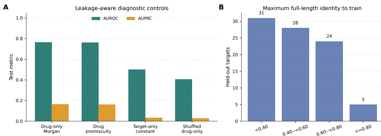
Figure 4. Diagnostic controls and target-relatedness audit. Panel A: leakage-aware controls on the exact-sequence-grouped cold-target test. Drug-only and drug-promiscuity scores use no target representation; the target-only constant is the only target-only control that does not use held-out target labels. Panel B: number of held-out targets by maximum full-length global sequence identity to any training target.
