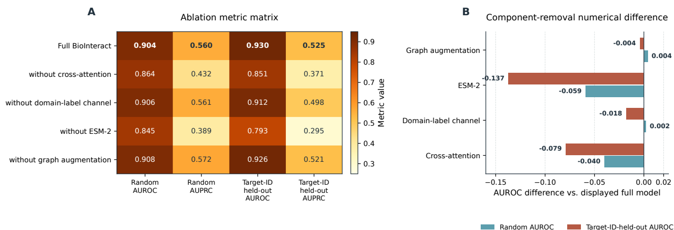
Figure 2. Component-removal summary. Panel A shows the random- and Target-ID-held-out metric matrix. Panel B reports each component-removed row’s AUROC difference from the displayed full-model row. Because the full-model row uses current canonical values while the component-removed rows retain their original numerical values, Panel B is descriptive rather than a controlled matched-retraining effect analysis. ESM-2 and cross-attention show the largest negative differences in both splits.
