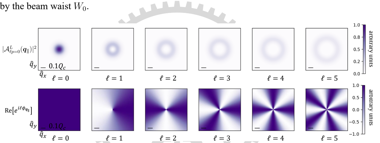
Figure 2.2 : Squared magnitude and phase distribution of \mathcal{A}_{\ell, p=0}^L(\mathbf{q}_{\parallel}) at z = 0 . The scale bar indicates the considered light-cone range for WSe 2 -monolayers, Q_c = 8.6 \mu\text{m}^{-1} .
