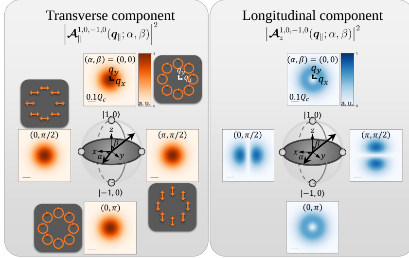
Figure 2.9 : Distribution (squared magnitude) of different components of \mathcal{A}_{\parallel}^{1,0,-1,0}(\mathbf{q}_{\parallel}; \alpha, \beta) on the Poincaré sphere, together with the corresponding polarization states of the transverse components. The scale bar indicates the considered 0.1 times light cone range, Q_c = 8.6 \mu\text{m}^{-1}
