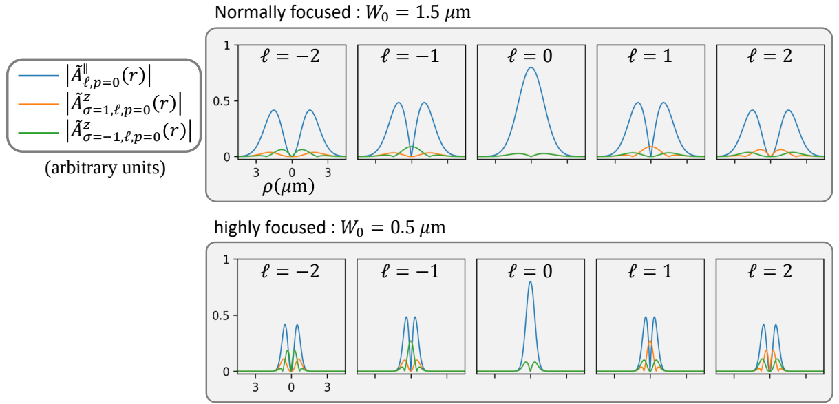
Figure 2.5 : Magnitude (absolute value) of \mathcal{A}_{\hat{\epsilon}, \ell, p=0}(\mathbf{r}) at z = 0 for different components and helicities. The \sigma\ell term leads to asymmetry between cases with the same \ell in the longitudinal component (a wavelength of 532 nm is assumed).
