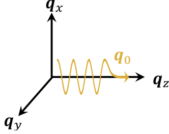
Figure 2.1 : Illustration of a dominant component of wavevector \mathbf{q}_0 lies along \hat{z}
