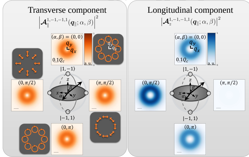
Figure 2.10 : Distribution (squared magnitude) of different components of \mathcal{A}_{\parallel}^{1,-1,-1,1}(\mathbf{q}_{\parallel}; \alpha, \beta) on the Poincaré sphere, together with the corresponding polarization states of the transverse components. The scale bar indicates the considered 0.1 times light cone range, Q_c = 8.6 \mu\text{m}^{-1}
