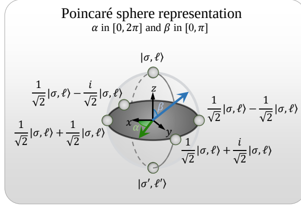
Figure 2.8 : The VVB state represented on the Poincaré sphere, parameterized by the azimuthal angle \alpha and polar angle \beta . Several representative combinations of \alpha and \beta are illustrated on the sphere surface as examples.
