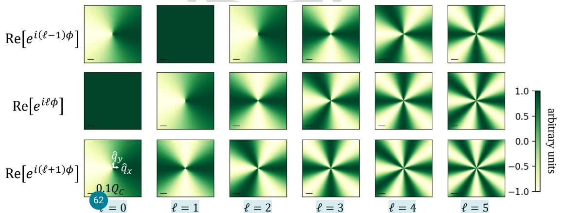
Figure 2.4 : Phase distribution of different components of \mathcal{A}_{\ell, p}^C(\mathbf{q}_{\parallel}) for different helicities. The scale bar indicates the considered 0.1 times light cone range for WSe 2 -monolayers, Q_c = 8.6 \mu\text{m}^{-1}
