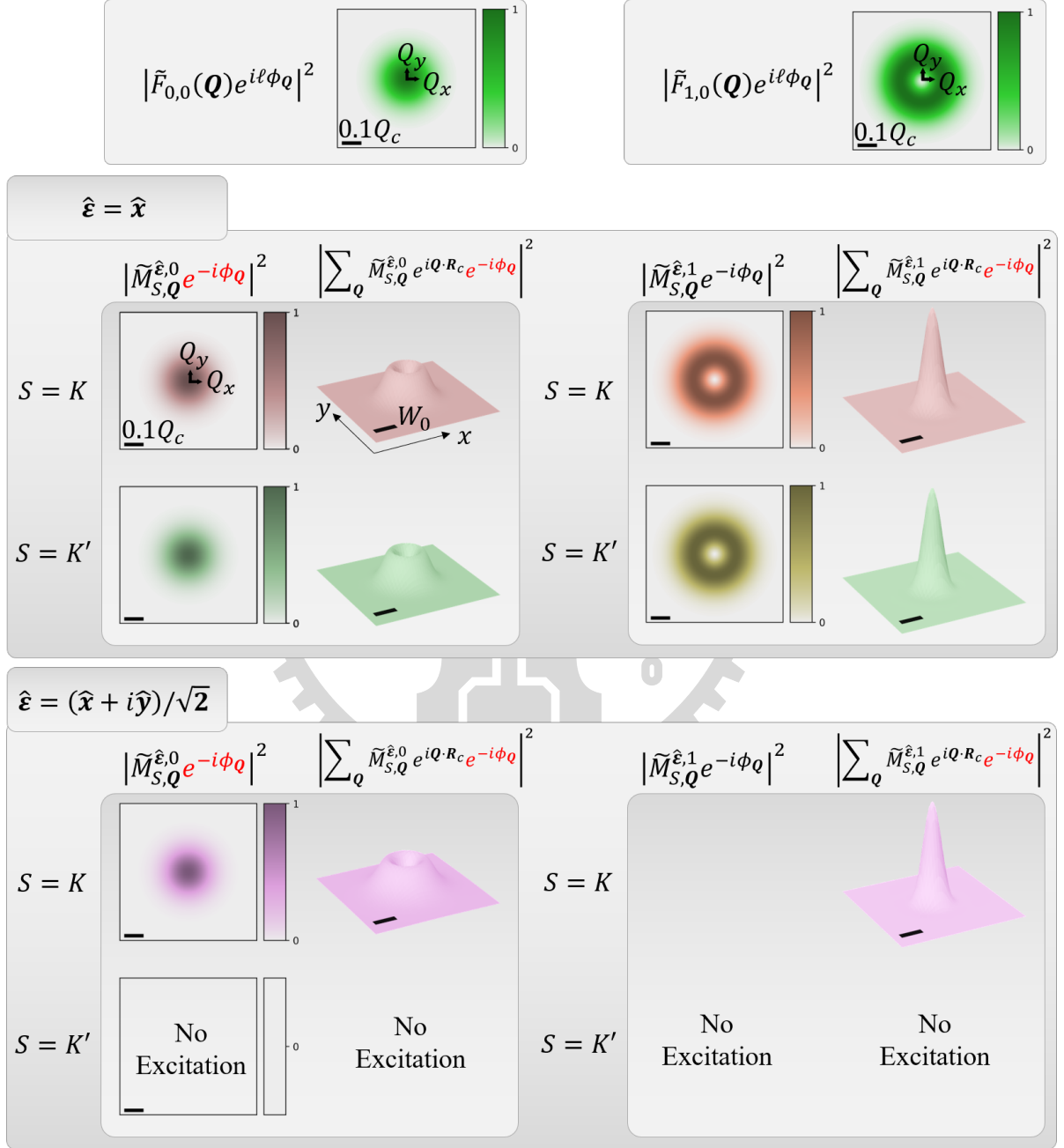
Figure 4.6 : Normalized squared magnitude distributions of the transverse component of the LG beam ( \ell = 0 and 1 ), together with the normalized squared magnitudes of the optical matrix element and the resulting valley exciton wave packet for different polarization unit vectors \hat{\varepsilon} . The scale bar indicates 0.1 times the light cone range for \text{WSe}_2 monolayers, Q_c = 8.6 \mu\text{m}^{-1} , and the beam waist is W_0 = 1.5 \mu\text{m}^{-1} .
