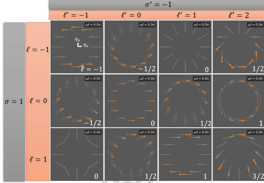
Figure 2.17 : Based on Eq. (2.48), polarization and instantaneous polarization distributions of \text{Re}[\tilde{\mathcal{A}}_{1,\ell,-1,\ell'}^{\parallel}(\mathbf{q}_{\parallel}, t; \alpha = 0, \beta = \frac{\pi}{2})] at \omega t = 0 , with \bar{\ell} indicated at the bottom right. Animation accessible via Figure 2.16.
