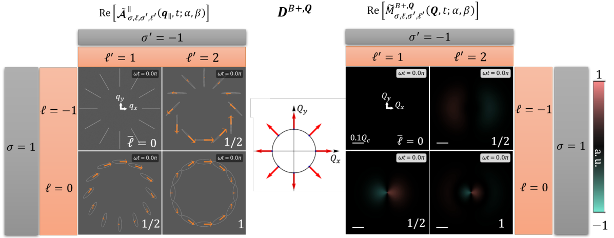
Figure 3.7 : Based on Eq. (2.48) and Eq. (3.15), distribution of \text{Re}[\tilde{\mathcal{A}}_{1, \ell, -1, \ell'}^{\parallel}(\mathbf{q}_{\parallel}, t; \alpha = 0, \beta = \frac{\pi}{2})] (left panel) and \text{Re}[\tilde{M}_{1, \ell, -1, \ell'}^{B+, \mathbf{Q}}(\mathbf{Q}, t; \alpha = 0, \beta = \frac{\pi}{2})] (right panel) at \omega t = 0 . The transition dipole moment for upper band BX is plotted in the middle. Animation accessible via Figure 3.5.
