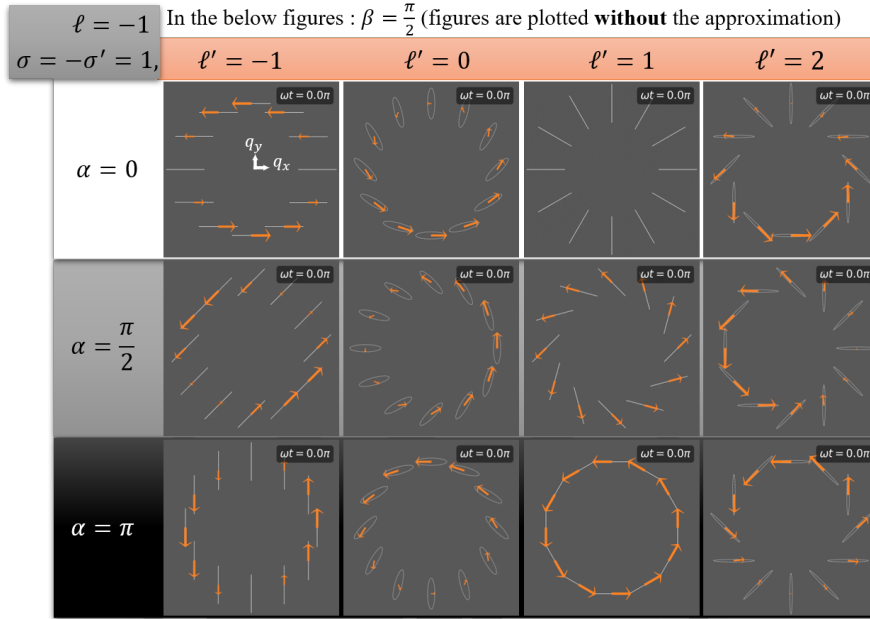
Figure 2.21 : Based on Eq. (2.48), polarization and instantaneous polarization distributions of \text{Re}[\tilde{\mathcal{A}}_{1,-1,-1,\ell'}(\mathbf{q}_{\parallel}, t; \alpha, \beta = \pi/2)] at \omega t = 0 for various \alpha . Animation accessible via Figure 2.20
