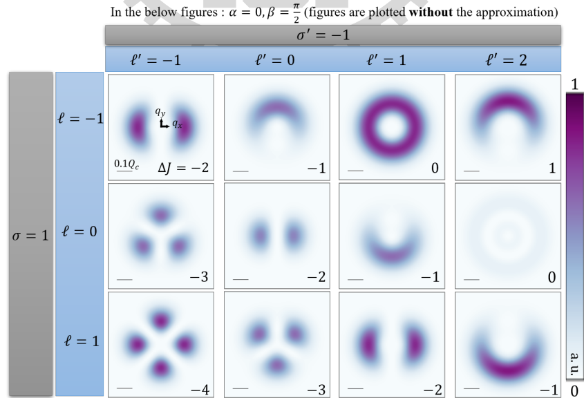
Figure 2.14 : Based on Eq. (2.44), distribution of \left| \tilde{\mathcal{A}}_{1,\ell,-1,\ell'}^z(\mathbf{q}_{\parallel}; \alpha = 0, \beta = \frac{\pi}{2}) \right|^2 , with \Delta J indicated at the bottom right.
