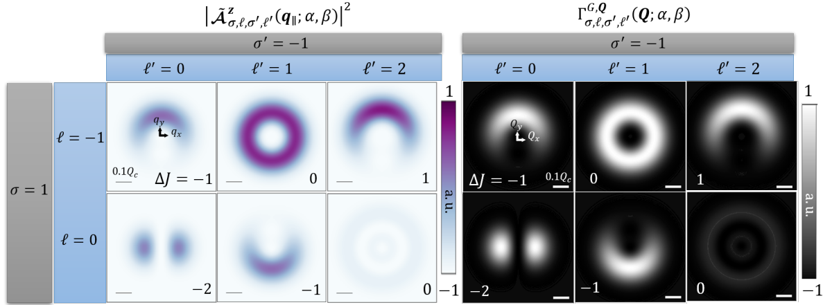
Figure 3.3 : Based on Eq. (2.44) and Eq. (3.10), distribution of |\tilde{\mathcal{A}}_{1, \ell, -1, \ell'}^z(\mathbf{q}_{\parallel}, t; \alpha = 0, \beta = \frac{\pi}{2})|^2 (left panel) and \Gamma_{\sigma, \ell, \sigma', \ell'}^{G, Q}(\mathbf{Q}; \alpha, \beta) (right panel), with \Delta J indicated at the bottom right.
