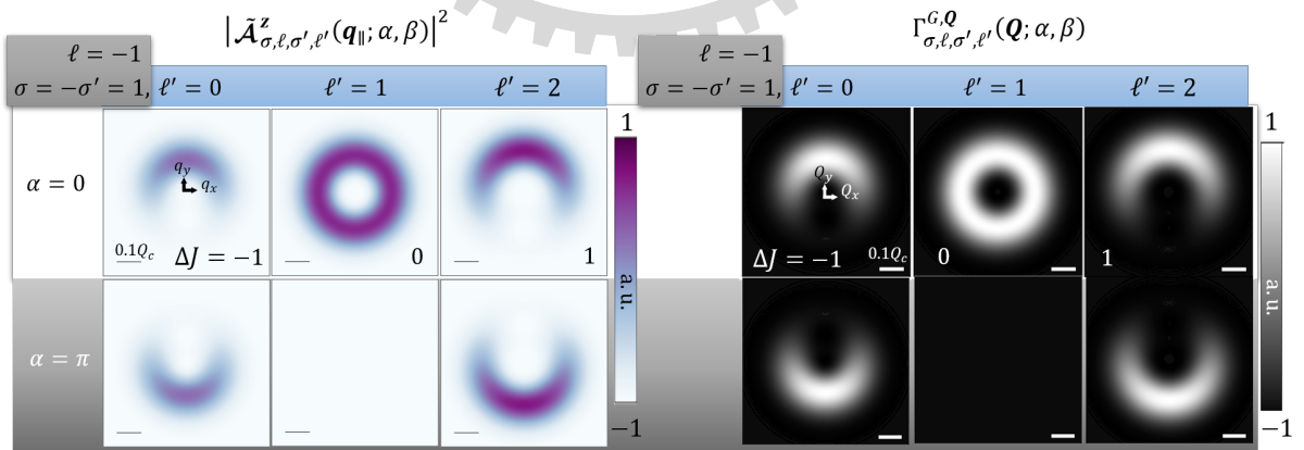
Figure 3.4 : Based on Eq. (2.44) and Eq. (3.10), distribution of |\tilde{\mathcal{A}}_{1, -1, -1, \ell'}^z(\mathbf{q}_{\parallel}, t; \alpha, \beta = \frac{\pi}{2})|^2 (left panel) and \Gamma_{\sigma, \ell, \sigma', \ell'}^{G, Q}(\mathbf{Q}; \alpha, \beta) (right panel), with -\frac{\alpha}{\Delta J} indicated at the bottom right.
