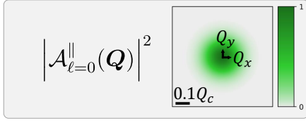
Figure 4.1 : Normalized squared magnitude distribution of the transverse component of the LG beam ( \ell = 0 ). The scale bar indicates 0.1 times the light cone range for WSe 2 monolayers, Q_c = 8.6 \mu\text{m}^{-1} .
