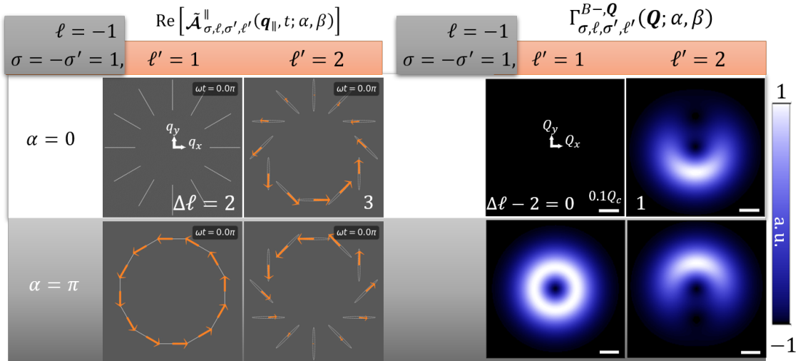
Figure 3.12 : Based on Eq. (2.48) and Eq. (3.16), distribution of \text{Re}[\tilde{\mathcal{A}}_{1, \ell, -1, \ell'}^{\parallel}(\mathbf{q}_{\parallel}, t; \alpha, \beta = \pi/2)] (left panel) and \Gamma_{\sigma, \ell, \sigma', \ell'}^{B-, Q}(\mathbf{Q}; \alpha, \beta = \pi/2) (right panel), with different \alpha . The transition dipole moment for lower band BX is plotted in the middle.
