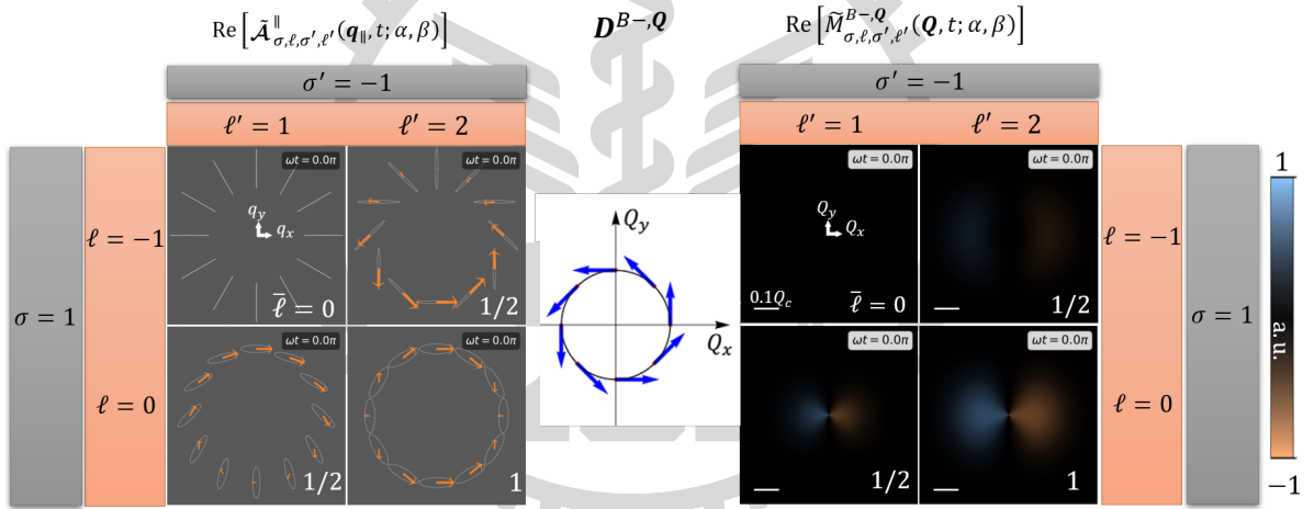
Figure 3.8 : Based on Eq. (2.48) and Eq. (3.16), distribution of \text{Re}[\tilde{\mathcal{A}}_{1, \ell, -1, \ell'}^{\parallel}(\mathbf{q}_{\parallel}, t; \alpha = 0, \beta = \frac{\pi}{2})] (left panel) and \text{Re}[\tilde{M}_{1, \ell, -1, \ell'}^{B-, \mathbf{Q}}(\mathbf{Q}, t; \alpha = 0, \beta = \frac{\pi}{2})] (right panel) at \omega t = 0 . The transition dipole moment for lower band BX is plotted in the middle. Animation accessible via Figure 3.6.
