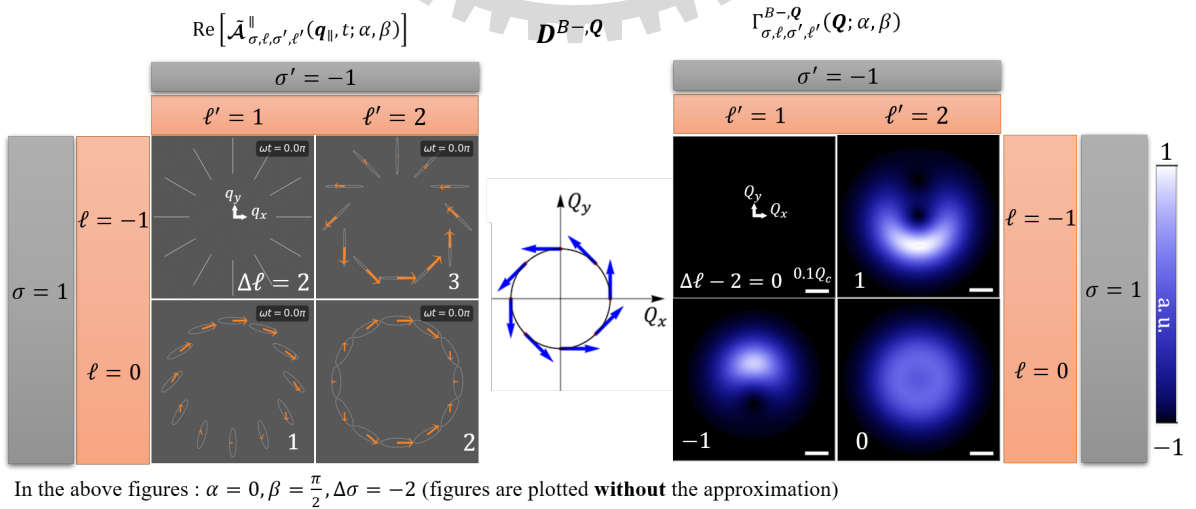
Figure 3.10 : Based on Eq. (2.48) and Eq. (3.16), distribution of \text{Re}[\tilde{\mathcal{A}}_{1,\ell,-1,\ell'}^{\parallel}(\mathbf{q}_{\parallel}, t; \alpha = 0, \beta = \frac{\pi}{2})] (left panel) and \Gamma_{\sigma,\ell,\sigma',\ell'}^{B-,Q}(\mathbf{Q}; \alpha = 0, \beta = \frac{\pi}{2}) (right panel), with \Delta\ell and \Delta\ell - 2 are indicated at the bottom. The transition dipole moment for lower band BX is plotted in the middle.
