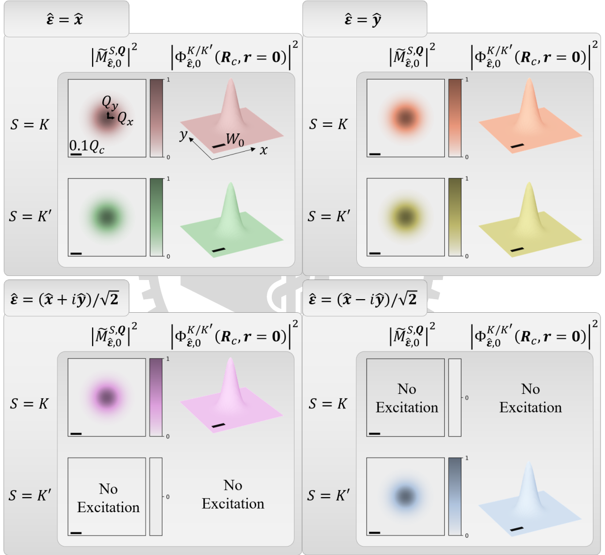
Figure 4.2 : Normalized squared magnitudes of the optical matrix element and the valley exciton wave packet excited by a LG beam ( \ell = 0 ) with different polarization unit vectors \hat{\varepsilon} . The scale bar indicates 0.1 Q_c , and the beam waist is W_0 = 1.5 \mu\text{m}^{-1} .
