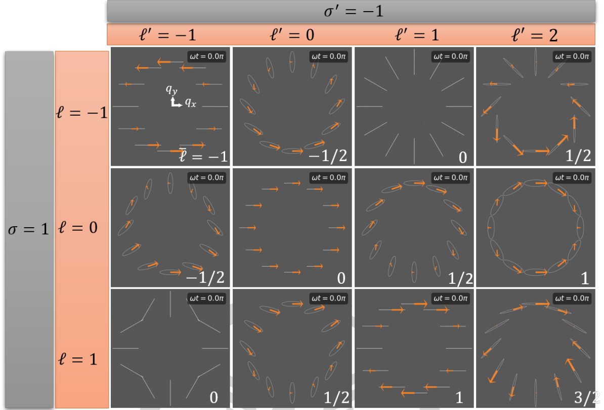
Figure 2.16 : Polarization, instantaneous polarization for the VVB \tilde{\mathcal{A}}_{1,\ell,-1,\ell'}^{\parallel}(\mathbf{q}_{\parallel}; \alpha = 0, \beta = \pi/2) , and the corresponding handedness of the elliptical polarization. \Delta\ell is indicated in the bottom right of each case, and those with an odd \Delta\ell are indicated by the red boxes. The notation used in the figure is illustrated in Figure 2.17.
