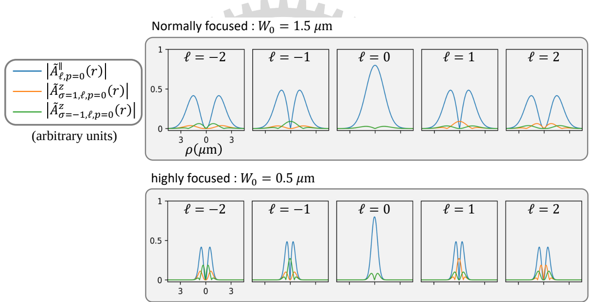
Figure 2.6 : Magnitude (absolute value) of \mathbf{A}_{\sigma,\ell,p=0}(\mathbf{r}) at z = 0 for different components and spin. The \sigma\ell term leads to asymmetry between cases with the same \ell in the longitudinal component (a wavelength of 532 nm is assumed).
