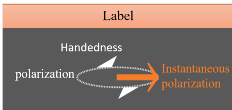
Figure 2.17 : Notation for Figure 2.16: dotted line (polarization), orange arrow ( t = 0 instantaneous polarization), triangles (elliptical handedness).
