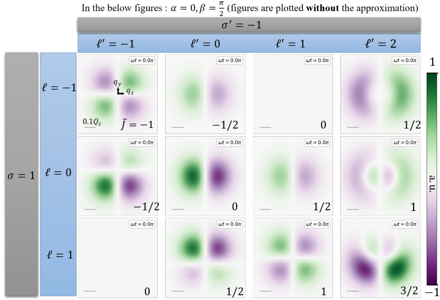
Figure 2.13 : Following Eq. (2.44), the distribution of \text{Re} \left[ \tilde{\mathcal{A}}_{1,\ell,-1,\ell'}^z(\mathbf{q}_{||}, t; \alpha = 0, \beta = \pi/2) \right] at \omega t = 0 . The animation can be viewed through the QR code in Figure 2.12.
