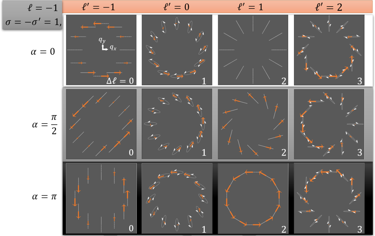
Figure 2.18 : Polarization, instantaneous polarization for the VVB \tilde{\mathcal{A}}_{1,-1,-1,\ell'}^{\parallel}(\mathbf{q}_{\parallel}; \alpha, \beta = \pi/2) , and the corresponding handedness of the elliptical polarization. The three different rows correspond to different \alpha settings. The notation used in the figure is illustrated in Figure 2.17.
