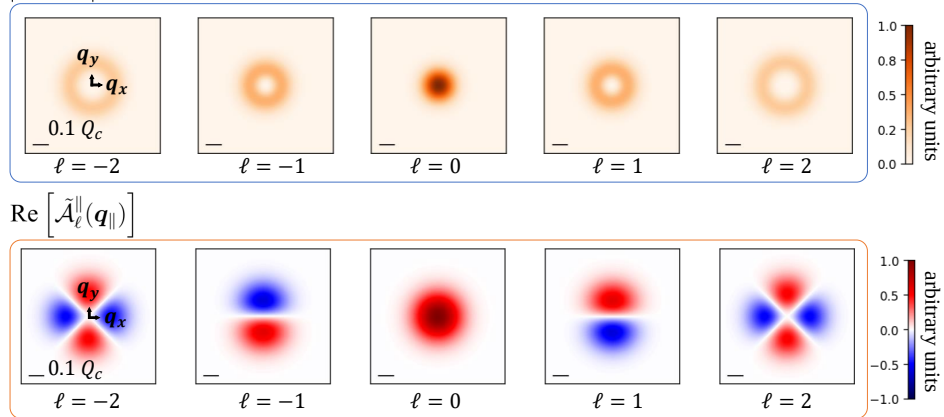
Figure 2.7 : Squared magnitude (intensity) and real part distribution of \tilde{\mathcal{A}}_{\ell}^{\parallel}(\mathbf{q}_{\parallel}) . The scale bar indicates 0.1 times the light-cone radius for WSe 2 monolayers, Q_c = 8.6 \mu\text{m}^{-1} .
