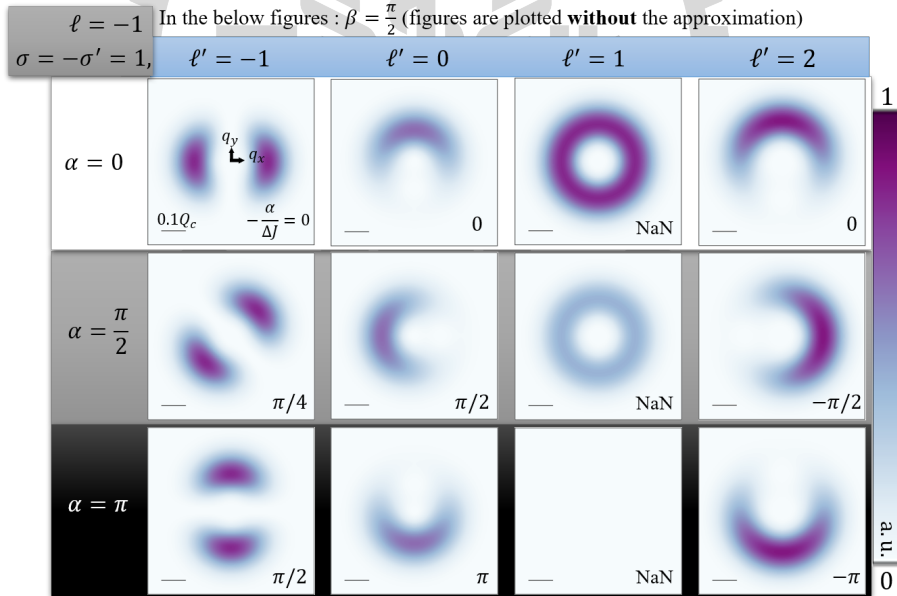
Figure 2.15 : Following Eq. (2.44), the distribution of \left| \tilde{\mathcal{A}}_{1,-1,-1,\ell'}^z(\mathbf{q}_{\parallel}, t; \alpha, \beta = \pi/2) \right|^2 with varying \alpha .
