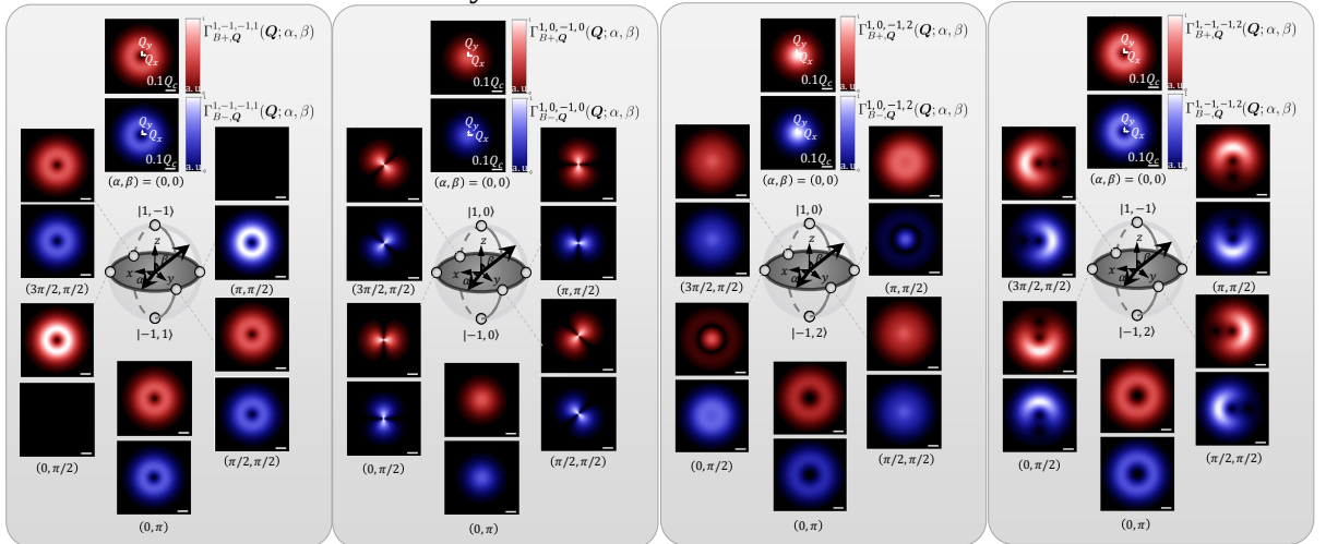
Figure 3.2 : Normalized transition rate of valley-mixed BXs excited by the VVB state |1, \ell, -1, \ell'; \alpha, \beta\rangle in center of mass momentum space. The scale bar indicates the considered 0.1 times light cone range for WSe 2 -monolayers, Q_c = 8.6 \mu\text{m}^{-1}
