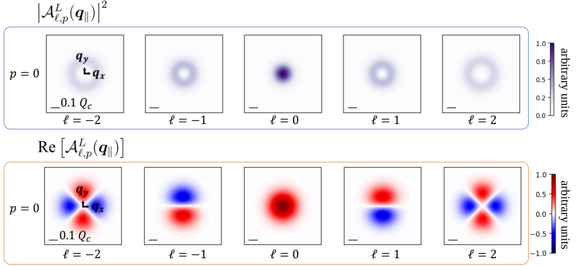
Figure 2.5 : Squared magnitude (intensity) and real part distribution of \mathcal{A}_{\ell,p=0}^L(\mathbf{q}_{\parallel}) . The scale bar indicates the considered 0.1 times light cone range for WSe 2 -monolayers, Q_c = 8.6 \mu\text{m}^{-1} .
