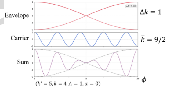
Figure 2.10: Example of a beating wave with \bar{k} = 9/2 at t = 0
