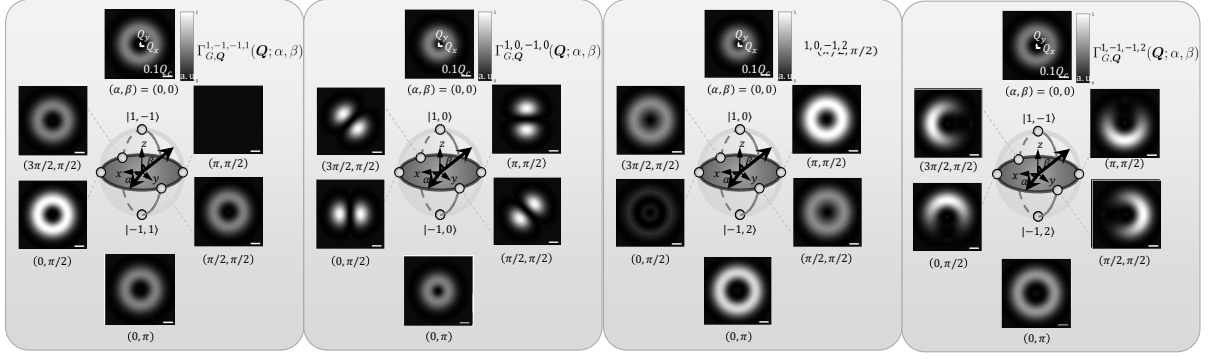
Figure 3.3 : Normalized transition rate of GXs excited by the VVB state |1, \ell, -1, \ell'; \alpha, \beta\rangle in center of mass momentum space. The scale bar indicates the considered 0.1 times light cone range for WSe 2 -monolayers, Q_c = 8.6 \mu\text{m}^{-1}
