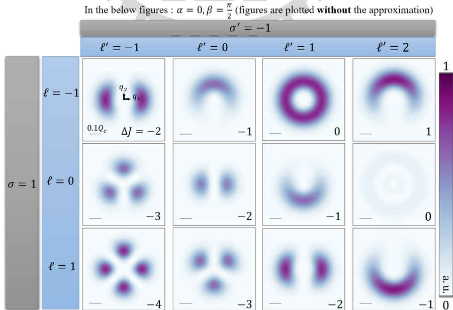
Figure 2.14 : Following Eq. (2.44), the distribution of \left| \tilde{\mathcal{A}}_{1,\ell,-1,\ell'}^z(\mathbf{q}_{||}, t; \alpha = 0, \beta = \pi/2) \right|^2 .
