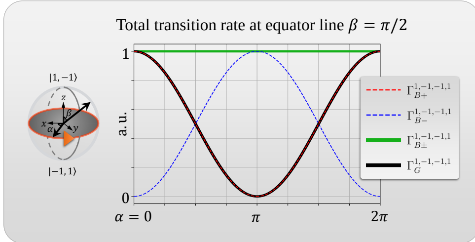
Figure 3.10 : Normalized total transition rates of BXs, total BXs, and GXs excited by a VVB state |1, -1, -1, 1; \alpha, \beta = \pi/2\rangle for azimuthal angles \alpha = 0 to 2\pi .
