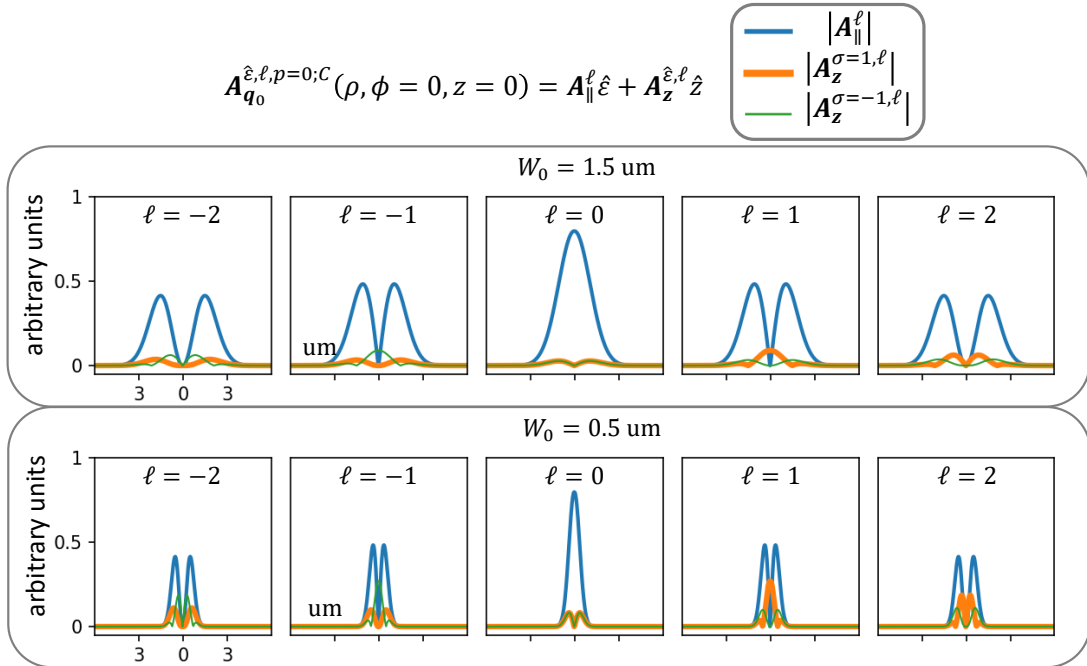
Figure 2.3 : Magnitude (absolute value) of \mathbf{A}_{q_0}^{\hat{\varepsilon}, \ell, p=0; C}(\mathbf{r}) at z = 0 for different components and helicities. The \sigma\ell term leads to asymmetry between cases with the same \ell in the longitudinal component (a wavelength of 532 \text{ nm} is assumed).
