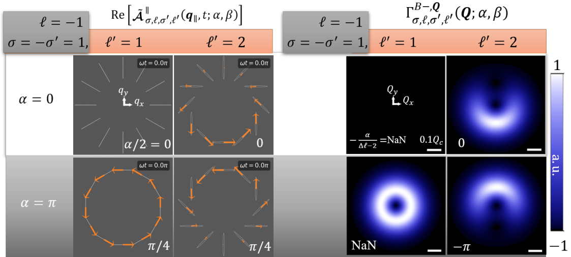
Figure 3.12 : Based on Eq. (2.47) and Eq. (3.16), distribution of \text{Re}[\tilde{\mathcal{A}}_{1, \ell, -1, \ell'}^{\parallel}(\mathbf{q}_{\parallel}, t; \alpha, \beta = \pi/2)] (left panel) and \Gamma_{\sigma, \ell, \sigma', \ell'}^{B-, Q}(\mathbf{Q}; \alpha, \beta = \pi/2) (right panel), with different \alpha . The transition dipole moment for lower band BX is plotted in the middle.
