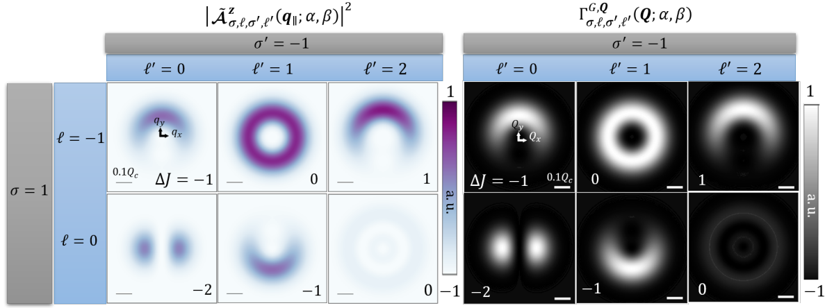
In the above figures : \alpha = 0, \beta = \frac{\pi}{2} (figures are plotted without the approximation)
