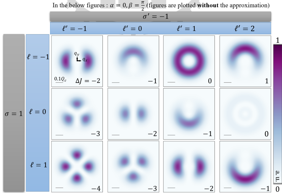
Figure 2.14 : Based on Eq. (2.44), distribution of \left| \tilde{\mathcal{A}}_{1,\ell,-1,\ell'}^z(\mathbf{q}_{\parallel}, t; \alpha = 0, \beta = \frac{\pi}{2}) \right|^2 , with \Delta J indicated at the bottom right.
