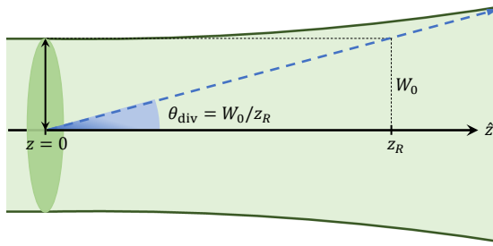
Figure 2.4 : Illustration of the beam-radius evolution and far-field divergence angle \theta_{\text{div}} .
