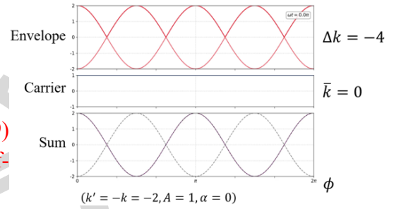
Figure 2.9: Example of a standing wave with \Delta k = -4 at t = 0 .
