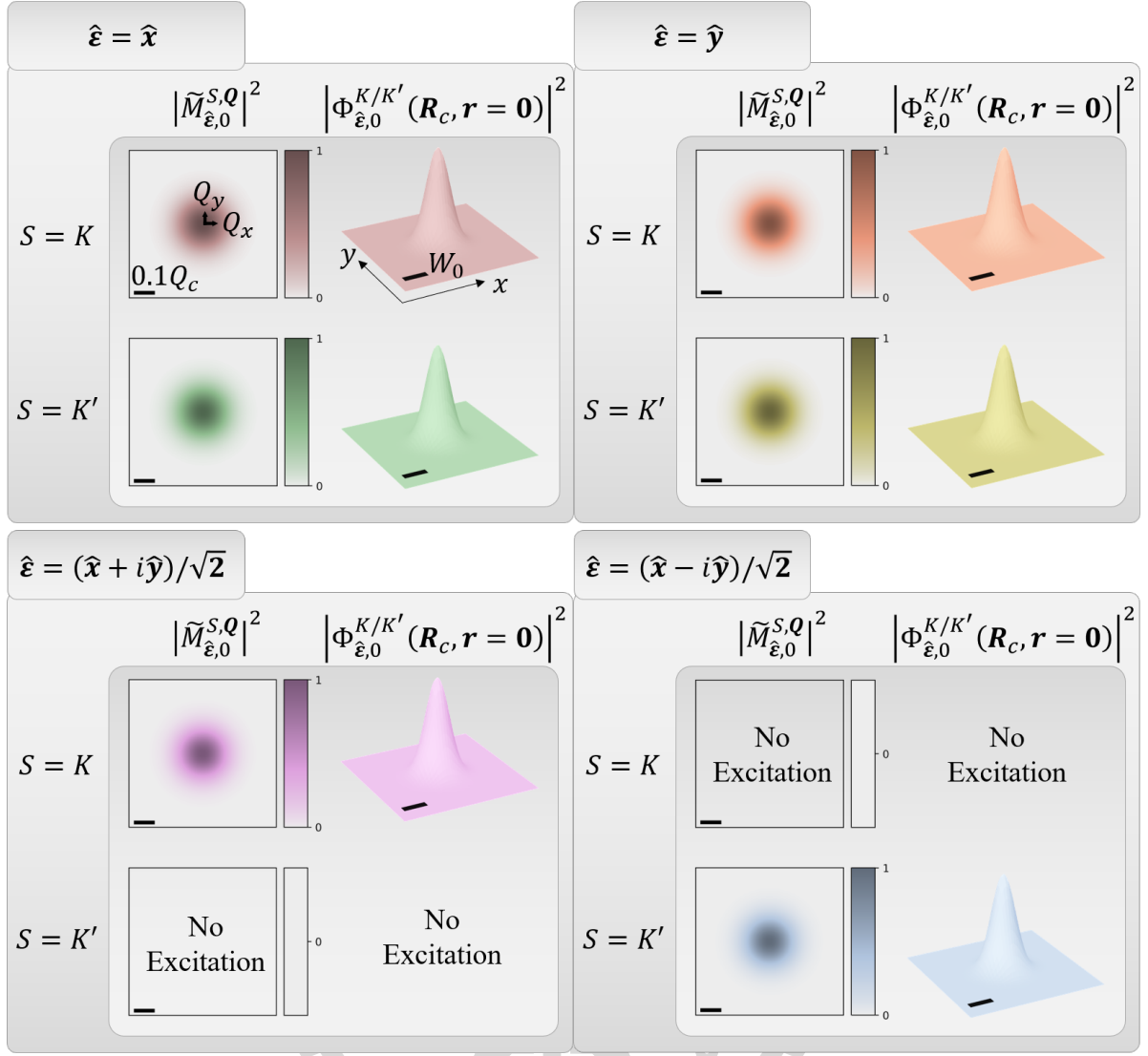
Figure 4.2 : Normalized squared magnitudes of the optical matrix element and the valley exciton wave packet excited by a LG beam ( \ell = 0 ) with different polarization unit vectors \hat{\epsilon} . The scale bar indicates 0.1 Q_c , and the beam waist is W_0 = 1.5 \mu\text{m}^{-1} .
