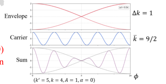
Figure 2.10: Example of a beating wave with \bar{k} = 9/2 at t = 0
