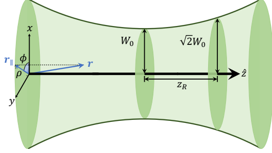
Figure 2.2 : Illustration of the evolution of the beam radius W(z) during propagation. The minimum beam radius W_0 occurs at the beam waist, and the Rayleigh range z_R is defined as the distance from the waist at which W(z_R) = \sqrt{2}W_0 .
