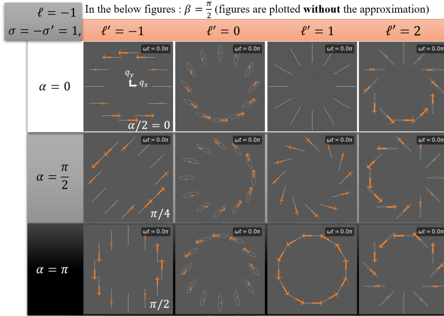
Figure 2.21 : Based on Eq. (2.47), polarization and instantaneous polarization distributions of \text{Re}[\tilde{\mathcal{A}}_{1,-1,-1,\ell'}(\mathbf{q}_{\parallel}, t; \alpha, \beta = \pi/2)] at \omega t = 0 for various \alpha . Animation accessible via Figure 2.20
