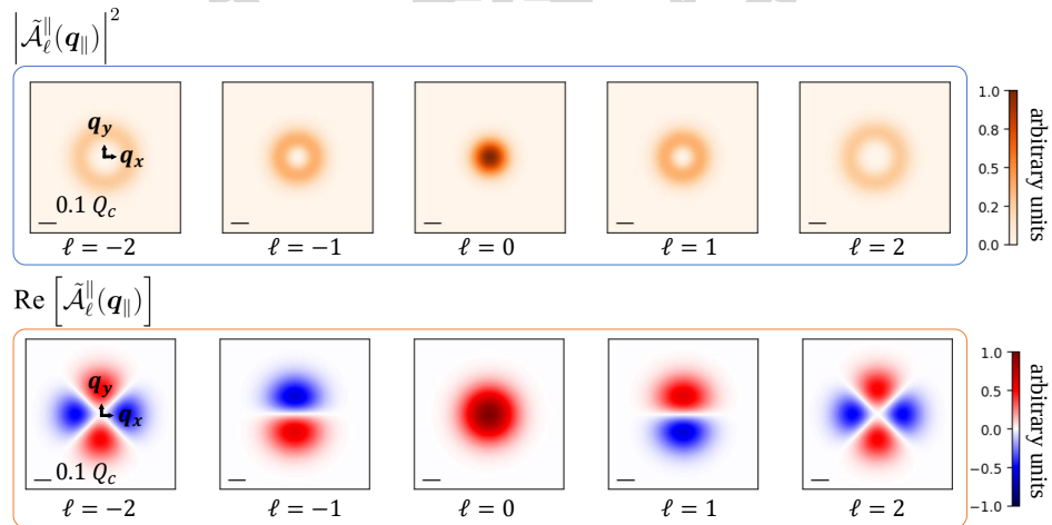
Figure 2.7 : Squared magnitude (intensity) and real part distribution of \tilde{\mathcal{A}}_{\ell}^{\parallel}(\mathbf{q}_{\parallel}) . The scale bar indicates 0.1 times the light-cone radius for WSe 2 monolayers, Q_c = 8.6 \mu\text{m}^{-1} .
