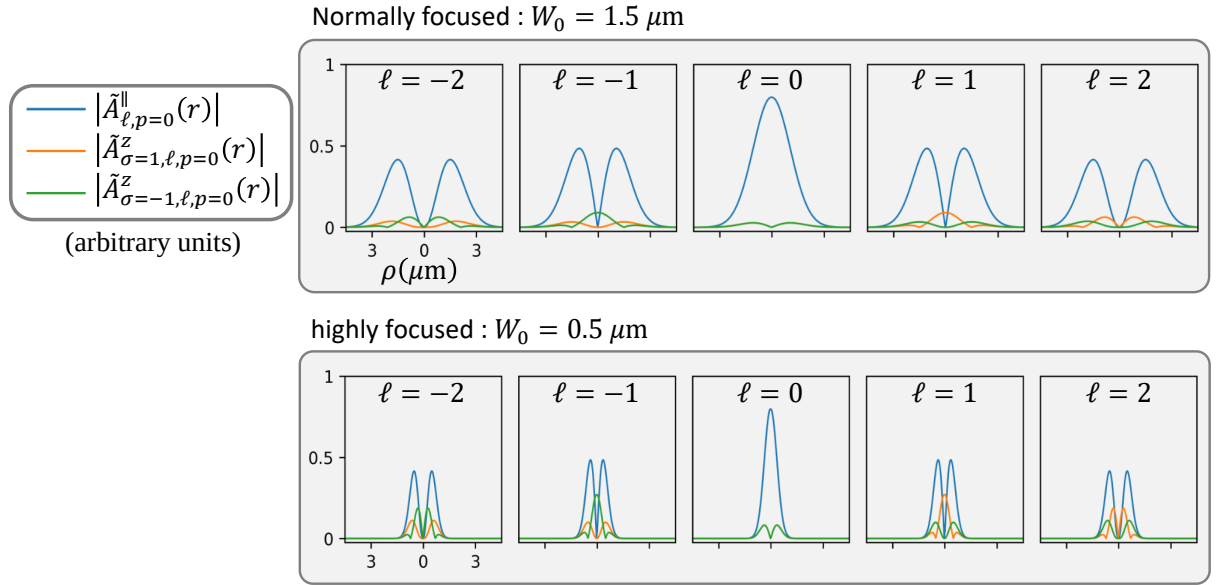
Figure 2.6 : Magnitude (absolute value) of \mathbf{A}_{\sigma,\ell,p=0}(\mathbf{r}) at z = 0 for different components and spin. The \sigma\ell term leads to asymmetry between cases with the same \ell in the longitudinal component (a wavelength of 532 nm is assumed).
