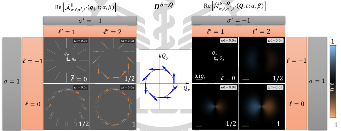
Figure 3.8 : Based on Eq. (2.47) and Eq. (3.16), distribution of \text{Re}[\tilde{\mathcal{A}}_{1, \ell, -1, \ell'}^{\parallel}(\mathbf{q}_{\parallel}, t; \alpha = 0, \beta = \frac{\pi}{2})] (left panel) and \text{Re}[\tilde{M}_{1, \ell, -1, \ell'}^{B-, \mathbf{Q}}(\mathbf{Q}, t; \alpha = 0, \beta = \frac{\pi}{2})] (right panel) at \omega t = 0 . The transition dipole moment for lower band BX is plotted in the middle. Animation accessible via Figure 3.6.
