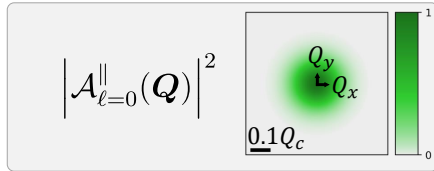
Figure 4.1 : Normalized squared magnitude distribution of the transverse component of the LG beam ( \ell = 0 ). The scale bar indicates 0.1 times the light cone range for WSe 2 monolayers, Q_c = 8.6 \mu\text{m}^{-1} .
