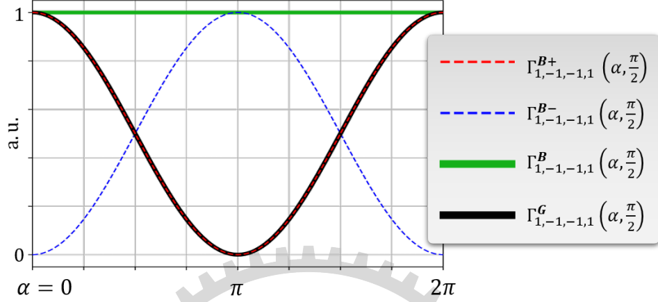
Figure 3.15 : Normalized total transition rates of BXs, total BXs, and GXs excited by a VVB with 1, -1, -1, 1 ; \alpha, \beta = \pi/2 for azimuthal angles \alpha = 0 to 2\pi .
