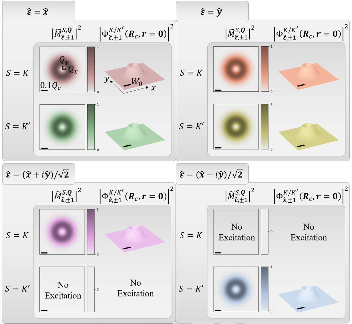
Figure 4.4 : Normalized squared magnitudes of the optical matrix element and the valley exciton wave packet excited by a LG beam ( \ell = 1 ) with different polarization unit vectors \hat{\epsilon} . The scale bar indicates 0.1 Q_c , and the beam waist is W_0 = 1.5 \mu\text{m}^{-1} .
