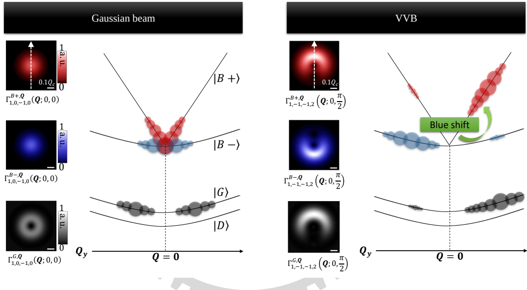
Figure 3.13 : Schematic of exciton population distribution along the Q_y axis for a VVB state ( \sigma, \ell, \sigma', \ell'=1, 0, -1, 0 ; \alpha = 0, \beta = 0 , Gaussian beam) and a VVB state ( \sigma, \ell, \sigma', \ell'=1, -1, -1, 2 ; \alpha = 0, \beta = \pi/2 ).
