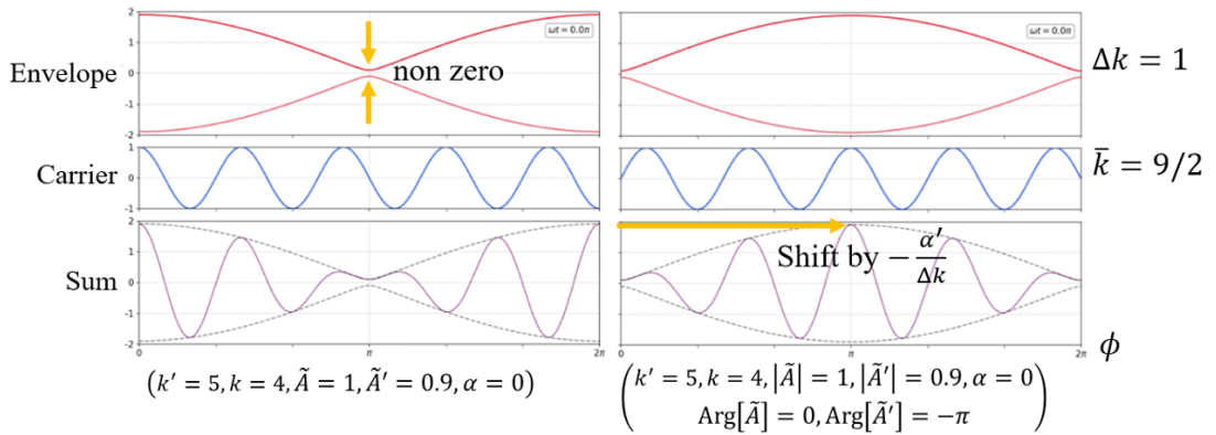
Figure 2.11 : Examples for mismatched amplitudes. The left(right) panel shows the case for real(complex) amplitude, where -\frac{\alpha'}{\Delta k} = \pi for the complex amplitude case.
