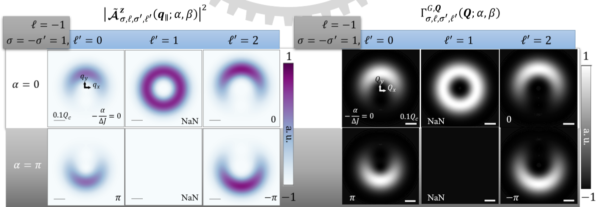
In the above figures : \beta = \frac{\pi}{2} (figures are plotted without the approximation)
