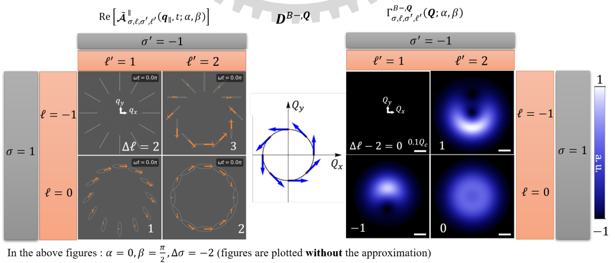
Figure 3.10 : Based on Eq. (2.47) and Eq. (3.16), distribution of \text{Re}[\tilde{\mathcal{A}}_{1,\ell,-1,\ell'}^{\parallel}(\mathbf{q}_{\parallel}, t; \alpha = 0, \beta = \frac{\pi}{2})] (left panel) and \Gamma_{\sigma,\ell,\sigma',\ell'}^{B-,Q}(\mathbf{Q}; \alpha = 0, \beta = \frac{\pi}{2}) (right panel), with \Delta\ell and \Delta\ell - 2 are indicated at the bottom. The transition dipole moment for lower band BX is plotted in the middle.
