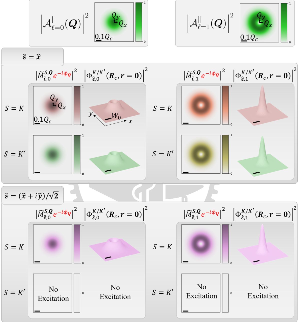
Figure 4.5 : Normalized squared magnitude distributions of the transverse component of the LG beam ( \ell = 0 and 1 ), together with the normalized squared magnitudes of the optical matrix element and the resulting valley exciton wave packet for different polarization unit vectors \hat{\epsilon} . The scale bar indicates 0.1 times the light cone range for WSe 2 monolayers, Q_c = 8.6 \mu\text{m}^{-1} , and the beam waist is W_0 = 1.5 \mu\text{m}^{-1} .
