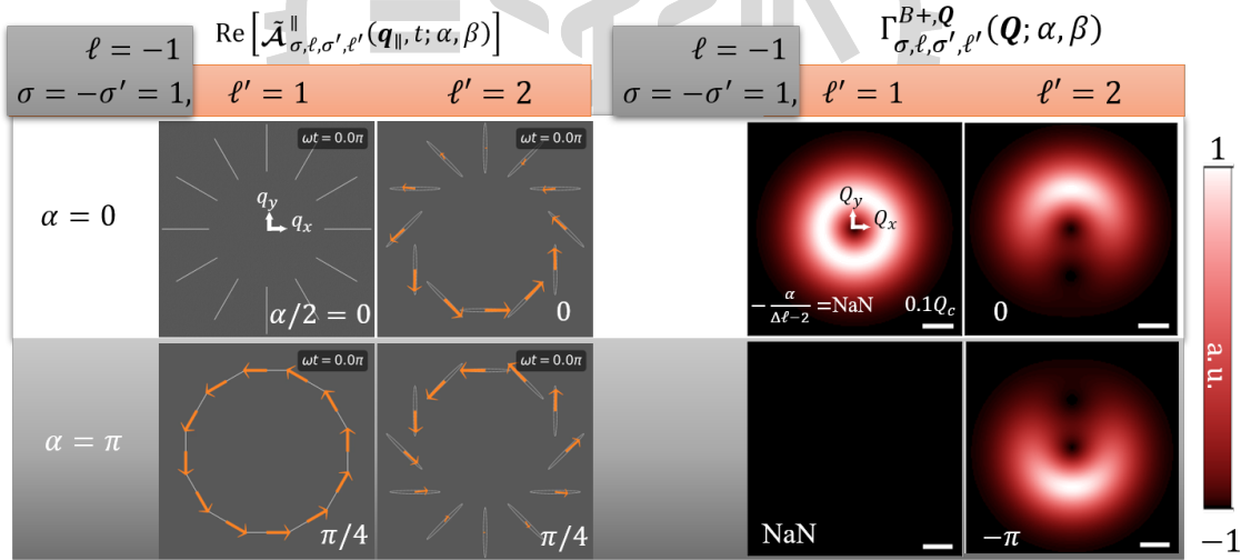
Figure 3.11 : Based on Eq. (2.47) and Eq. (3.15), distribution of \text{Re}[\tilde{\mathcal{A}}_{1, \ell, -1, \ell'}^{\parallel}(\mathbf{q}_{\parallel}, t; \alpha, \beta = \pi/2)] (left panel) and \Gamma_{\sigma, \ell, \sigma', \ell'}^{B+,Q}(\mathbf{Q}; \alpha, \beta = \pi/2) (right panel), with different \alpha . The transition dipole moment for upper band BX is plotted in the middle.
