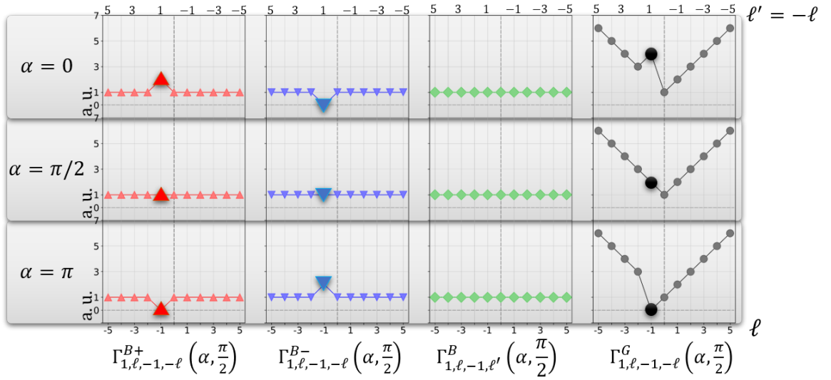
Figure 3.14 : Normalized total transition rates of BXs, total BXs, and GX excited by a VVB with \sigma, \ell, \sigma', \ell' = 1, \ell, -1, -\ell , with \beta = \pi/2 and varying \ell and \alpha .
