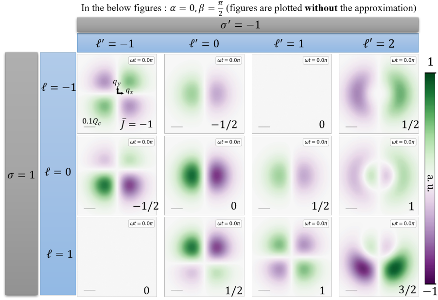
Figure 2.13 : Based on Eq. (2.44), distribution of \text{Re}[\tilde{\mathcal{A}}_{1,\ell,-1,\ell'}^z(\mathbf{q}_{\parallel}, t; \alpha = 0, \beta = \frac{\pi}{2})] at \omega t = 0 , with \bar{J} indicated at the bottom right. Animation accessible via Figure 2.12.
