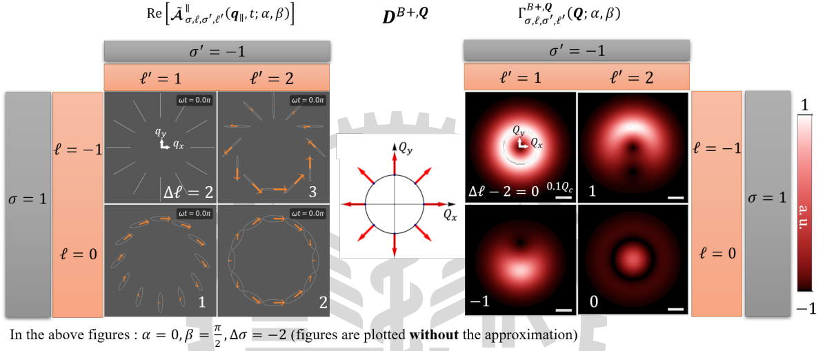
Figure 3.9 : Based on Eq. (2.47) and Eq. (3.15), distribution of \text{Re}[\tilde{\mathcal{A}}_{1,\ell,-1,\ell'}^{\parallel}(\mathbf{q}_{\parallel}, t; \alpha = 0, \beta = \frac{\pi}{2})] (left panel) and \Gamma_{\sigma,\ell,\sigma',\ell'}^{B+,Q}(\mathbf{Q}; \alpha = 0, \beta = \frac{\pi}{2}) (right panel), with \Delta\ell and \Delta\ell - 2 are indicated at the bottom. The transition dipole moment for upper band BX is plotted in the middle.
