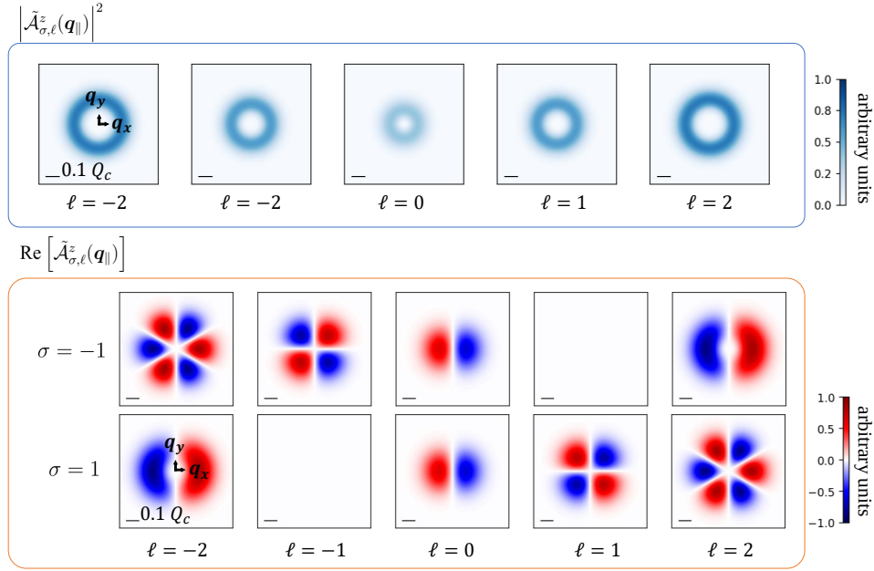
Figure 2.8 : Squared magnitude (intensity) and real part distribution of \tilde{\mathcal{A}}_{\sigma,\ell}^z(\mathbf{q}_{||}) . The scale bar indicates 0.1 times the light-cone radius for WSe 2 monolayers, Q_c = 8.6 \mu\text{m}^{-1} .
