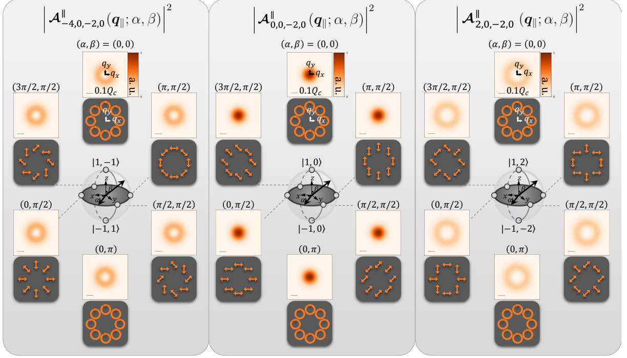
Figure 2.8 : Squared magnitude and polarization distribution of \mathcal{A}_{-2\ell,0,-2,0}^{\parallel}(\mathbf{q}_{\parallel}; \alpha, \beta) . The corresponding VVB states are represented on the Poincaré sphere, where the north and south poles correspond to the basis states |\sigma, \ell\rangle and |\sigma', \ell'\rangle , respectively.
