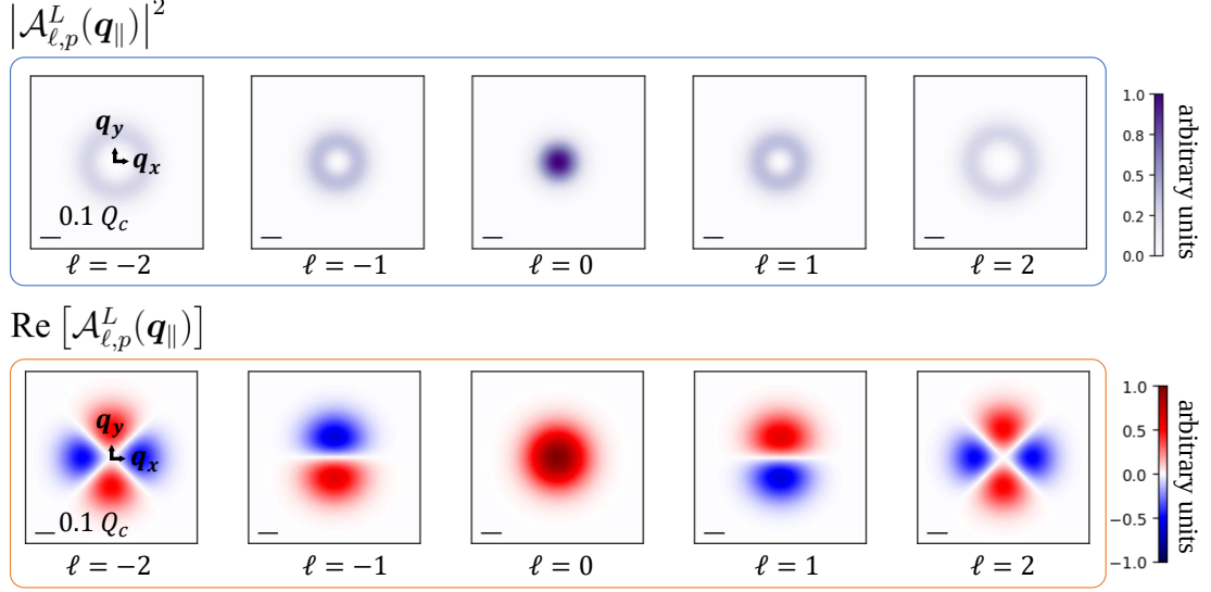
Figure 2.4 : Squared magnitude (intensity) and real part distribution of \mathcal{A}_{\ell,p=0}^L(\mathbf{q}_{||}) . The scale bar indicates the considered 0.1 times light cone range for WSe 2 -monolayers, Q_c = 8.6 \mu\text{m}^{-1} .
