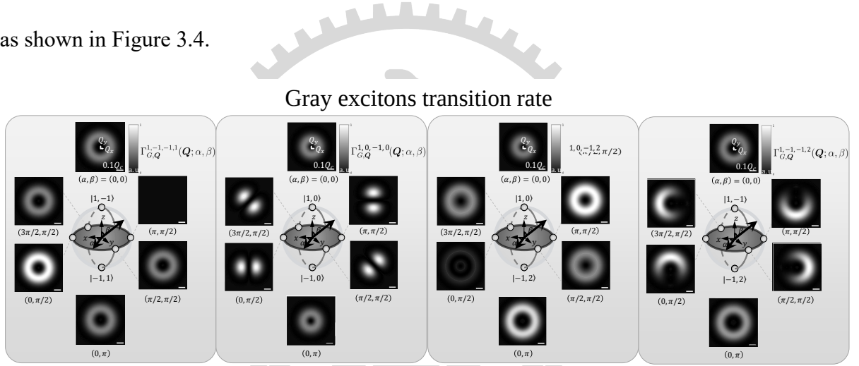
Figure 3.4 : Normalized transition rate of GXs excited by the VVB state |1, -1, -1, 1; \alpha, \beta\rangle in momentum space.
