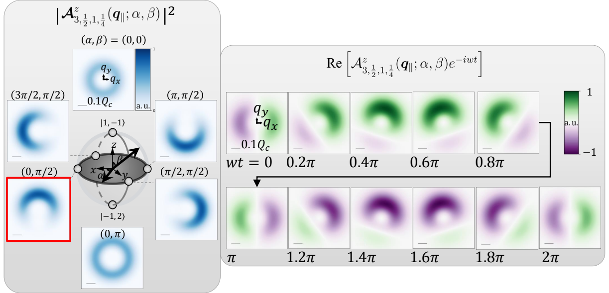
Figure 2.10 : Squared magnitude of \mathcal{A}_{3, \frac{1}{2}, 1, \frac{1}{4}}^z(\mathbf{q}_{\parallel}; \alpha, \beta) together with the time-dependent real part for the case (\alpha = 0, \beta = \pi/2) . The corresponding VVB states are represented on the Poincaré sphere.
