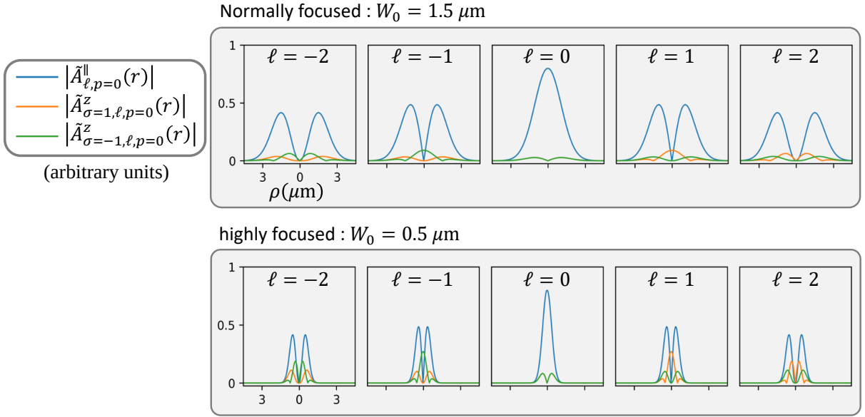
Figure 2.5 : Magnitude (absolute value) of \tilde{\mathcal{A}}_{\sigma,\ell,p=0}(\mathbf{r}) at z = 0 for different components and spin. The \sigma\ell term leads to asymmetry between cases with the same \ell in the longitudinal component (a wavelength of 532 nm is assumed).
