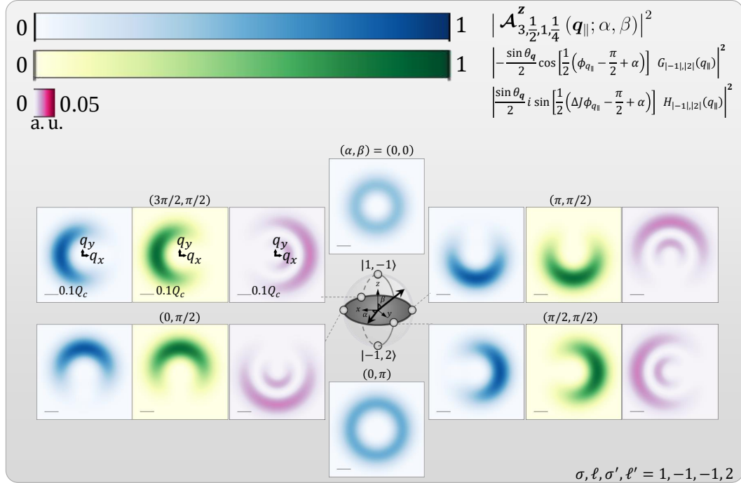
Figure 2.9 : Squared magnitude of \mathcal{A}_{3, \frac{1}{2}, 1, \frac{1}{4}}^z(\mathbf{q}_{\parallel}; \alpha, \beta) (blue) along with two of its components (green/magenta). The corresponding VVB states are represented on the Poincaré sphere.
