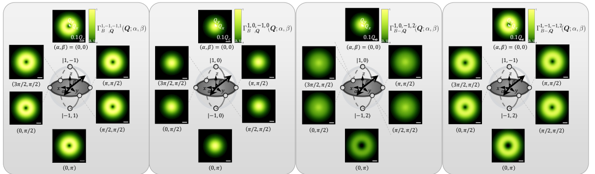
Figure 3.3 : Normalized transition rate of total BXs excited by the VVB state |1, -1, -1, 1; \alpha, \beta\rangle in momentum space.
