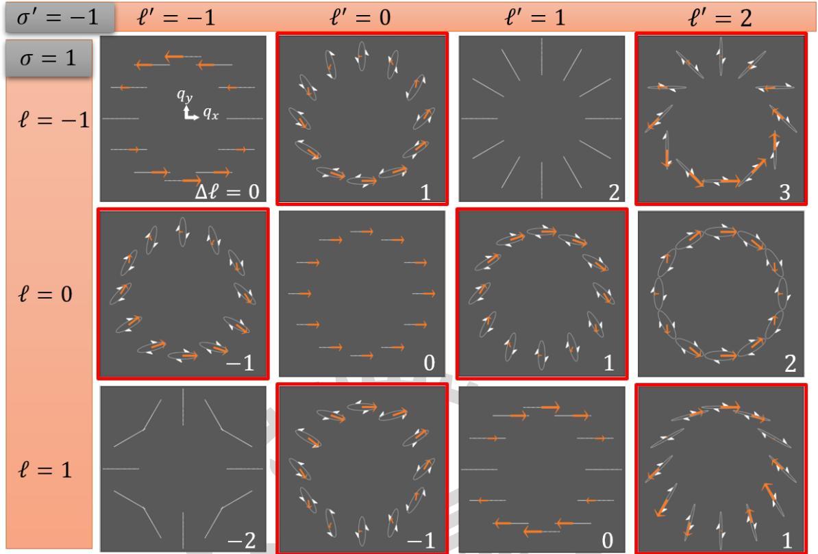
Figure 2.12 : Polarization, instantaneous polarization for the VVB \tilde{\mathcal{A}}_{1,\ell,-1,\ell'}^{\parallel}(\mathbf{q}_{\parallel}; \alpha = 0, \beta = \pi/2) , and the corresponding handedness of the elliptical polarization. \Delta\ell is indicated in the bottom right of each case, and those with an odd \Delta\ell are indicated by the red boxes. The notation used in the figure is illustrated in Figure 2.13.
