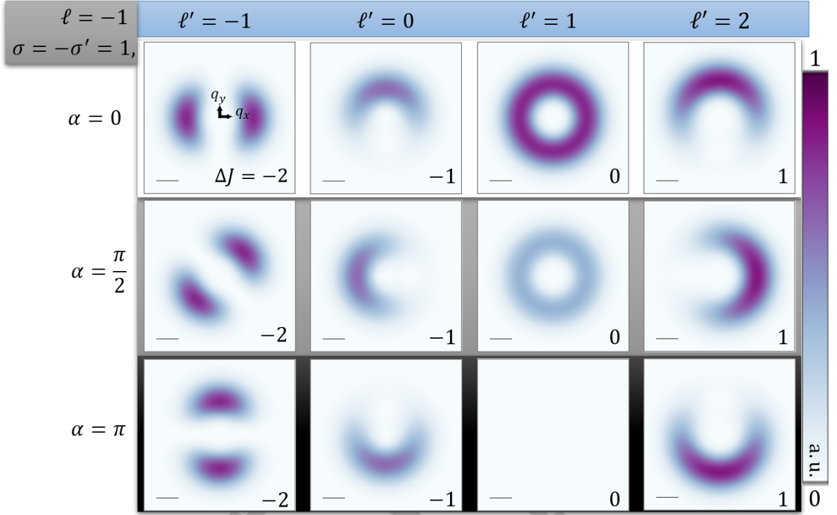
Figure 2.16 : Intensity of the longitudinal component of a VVB, \tilde{\mathcal{A}}_{1,-1,-1,\ell'}^z(\mathbf{q}_{\parallel}; \alpha, \beta = \pi/2) . The three rows correspond to different values of \alpha . The intensity scale has been standardized according to the colorbar on the right.
