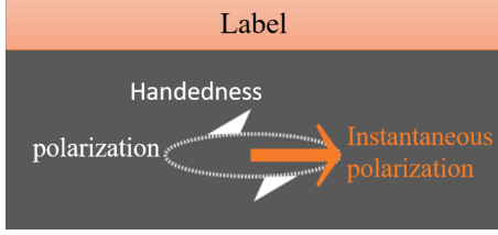
Figure 2.13 : Notation for Figure 2.12: dotted line (polarization), orange arrow ( t = 0 instantaneous polarization), triangles (elliptical handedness).
