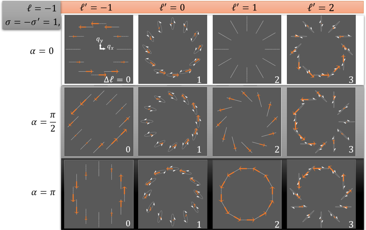
Figure 2.14 : Polarization, instantaneous polarization for the VVB \tilde{\mathcal{A}}_{1,-1,-1,\ell'}^{\parallel}(\mathbf{q}_{\parallel}; \alpha, \beta = \pi/2) , and the corresponding handedness of the elliptical polarization. The three different rows correspond to different \alpha settings. The notation used in the figure is illustrated in Figure 2.13.
