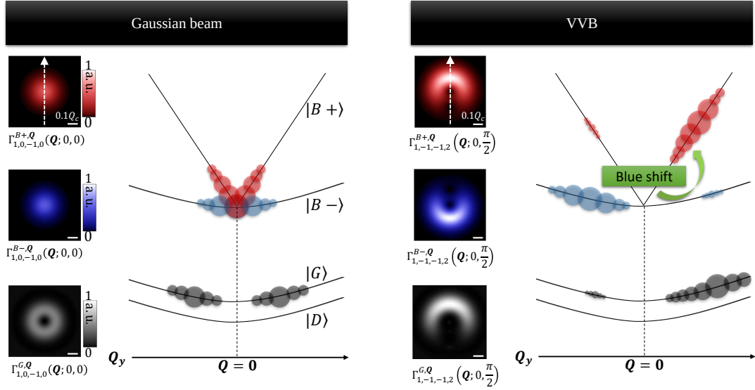
Figure 3.13 : Schematic of exciton population distribution along the Q_y axis for a VVB state ( \sigma, \ell, \sigma', \ell'=1, 0, -1, 0; \alpha = 0, \beta = 0 , Gaussian beam) and a VVB state ( \sigma, \ell, \sigma', \ell'=1, -1, -1, 2; \alpha = 0, \beta = \pi/2 ).
