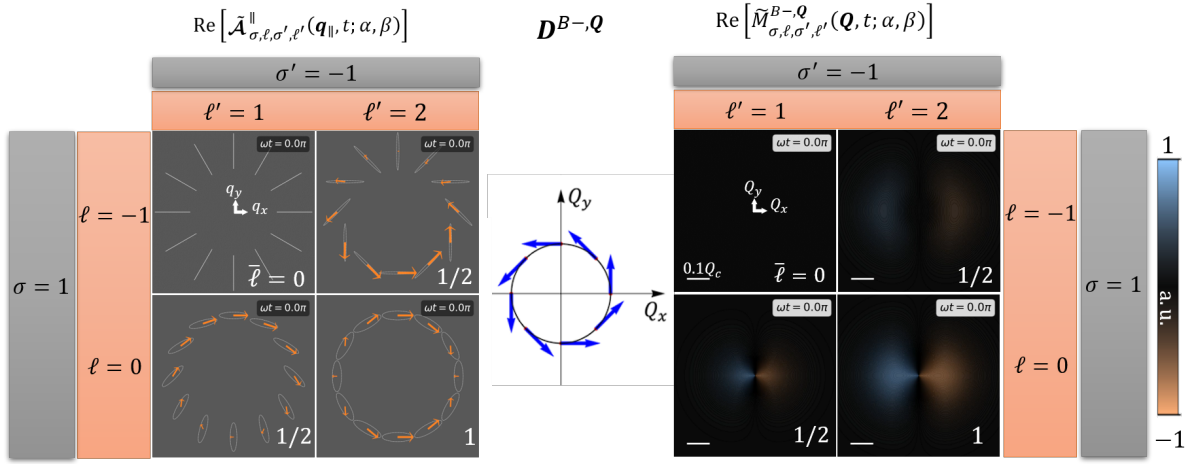
In the above figures : \alpha = 0, \beta = \frac{\pi}{2}, \Delta\sigma = -2 (figures are plotted without the approximation)
