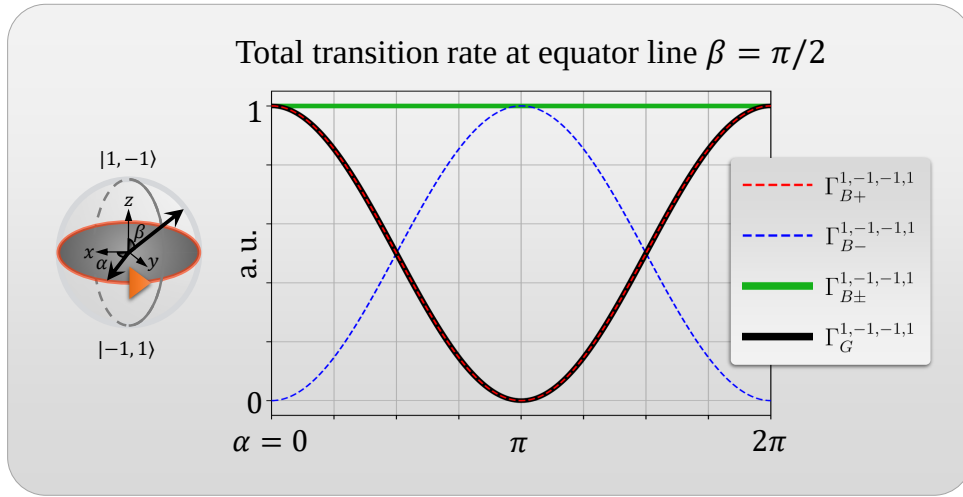
Figure 3.15 : Normalized total transition rates of BXs, total BXs, and GXs excited by a VVB state |1, -1, -1, 1; \alpha, \beta = \pi/2\rangle for azimuthal angles \alpha = 0 to 2\pi .
