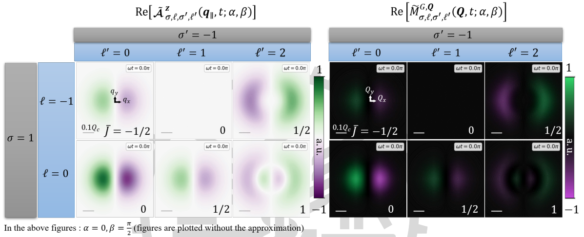
Figure 3.2 : Based on Eq. (2.44) and Eq. (3.10), distribution of \text{Re}[\tilde{\mathcal{A}}_{1,\ell,-1,\ell'}^z(q_{||}, t; \alpha = 0, \beta = \frac{\pi}{2})] (left panel) and \text{Re}[\tilde{M}_{1,\ell,-1,\ell'}^{G,Q}(Q, t; \alpha = 0, \beta = \frac{\pi}{2})] (right panel) at \omega t = 0 , with \bar{J} indicated at the bottom right. Animation accessible via Figure 3.1.
