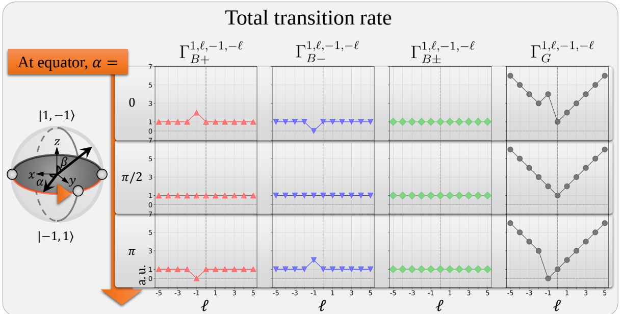
Figure 3.14 : Normalized total transition rates of BXs, total BXs, and GX excited by a VVB state |1, \ell, -1, -\ell; \alpha, \beta = \pi/2\rangle , for \ell \in \mathbb{Z} with \ell \in [-5, 5] , and for azimuthal angles \alpha = 0, \pi/2, \pi .
