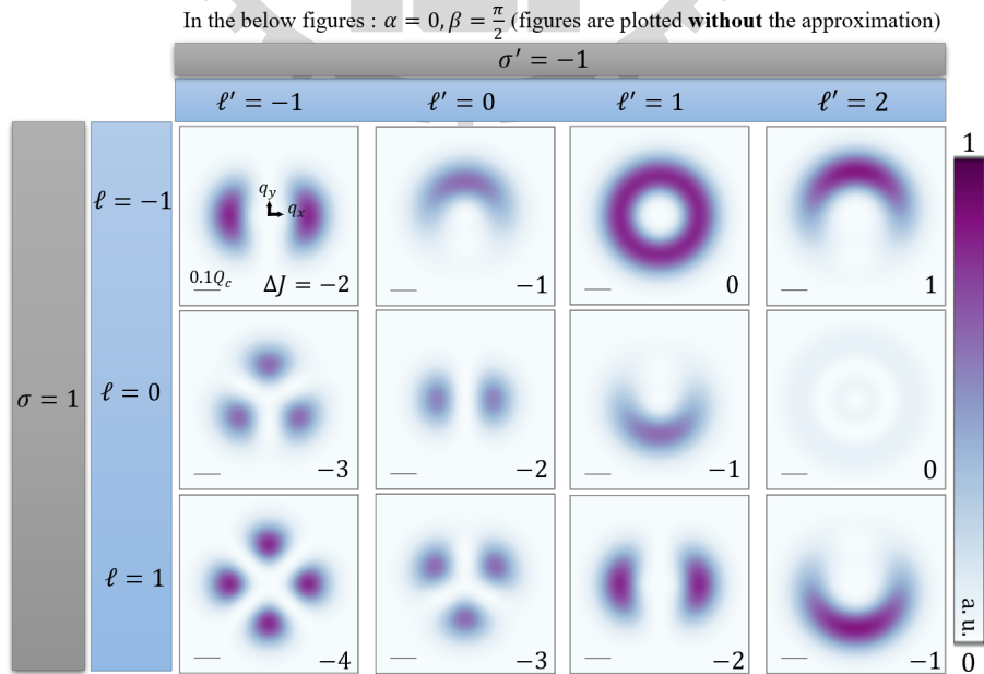
Figure 2.14 : Based on Eq. (2.44), distribution of \left| \tilde{\mathcal{A}}_{1, \ell, -1, \ell'}^z(\mathbf{q}_{\parallel}, t; \alpha = 0, \beta = \frac{\pi}{2}) \right|^2 , with \Delta J indicated at the bottom right.
