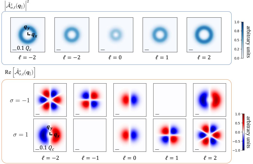
Figure 2.7 : Squared magnitude (intensity) and real part distribution of \tilde{\mathcal{A}}_{\sigma,\ell}^z(\mathbf{q}_{||}) . The scale bar indicates 0.1 times the light-cone radius for WSe 2 monolayers, Q_c = 8.6 \mu\text{m}^{-1} .
