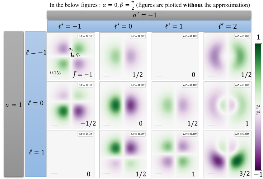
Figure 2.13 : Based on Eq. (2.44), distribution of \text{Re}[\tilde{\mathcal{A}}_{1, \ell, -1, \ell'}^z(\mathbf{q}_{\parallel}, t; \alpha = 0, \beta = \frac{\pi}{2})] at \omega t = 0 , with \bar{J} indicated at the bottom right. Animation accessible via Figure 2.12.
