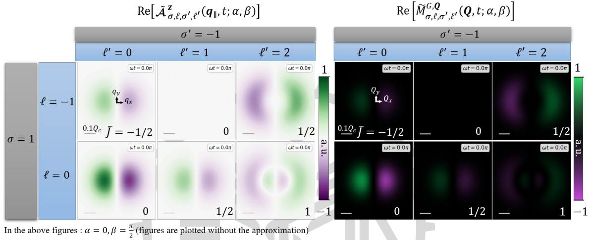
Figure 3.2 : Based on Eq. (2.44) and Eq. (3.10), distribution of \text{Re}[\tilde{\mathcal{A}}_{1,\ell,-1,\ell'}^z(\mathbf{q}_{||}, t; \alpha = 0, \beta = \frac{\pi}{2})] (left panel) and \text{Re}[\tilde{M}_{1,\ell,-1,\ell'}^{G,Q}(\mathbf{Q}, t; \alpha = 0, \beta = \frac{\pi}{2})] (right panel) at \omega t = 0 , with \bar{J} indicated at the bottom right. Animation accessible via Figure 3.1.
