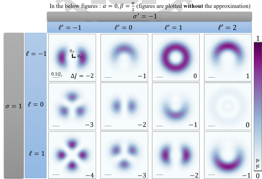
Figure 2.14 : Based on Eq. (2.44), distribution of |\tilde{\mathcal{A}}_{1, \ell, -1, \ell'}^z(\mathbf{q}_{\parallel}; \alpha = 0, \beta = \frac{\pi}{2})|^2 , with \Delta J indicated at the bottom right.
