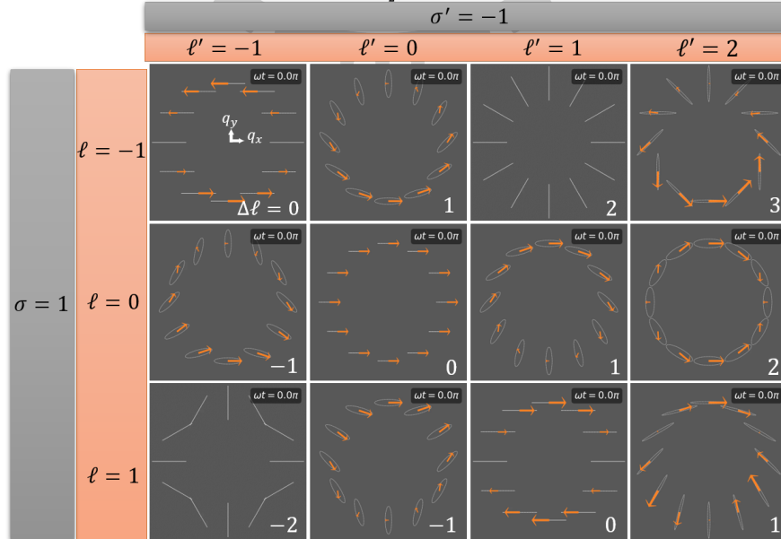
Figure 2.19 : Same figure as Figure 2.17 but denoted with \Delta\ell at the bottom right.
