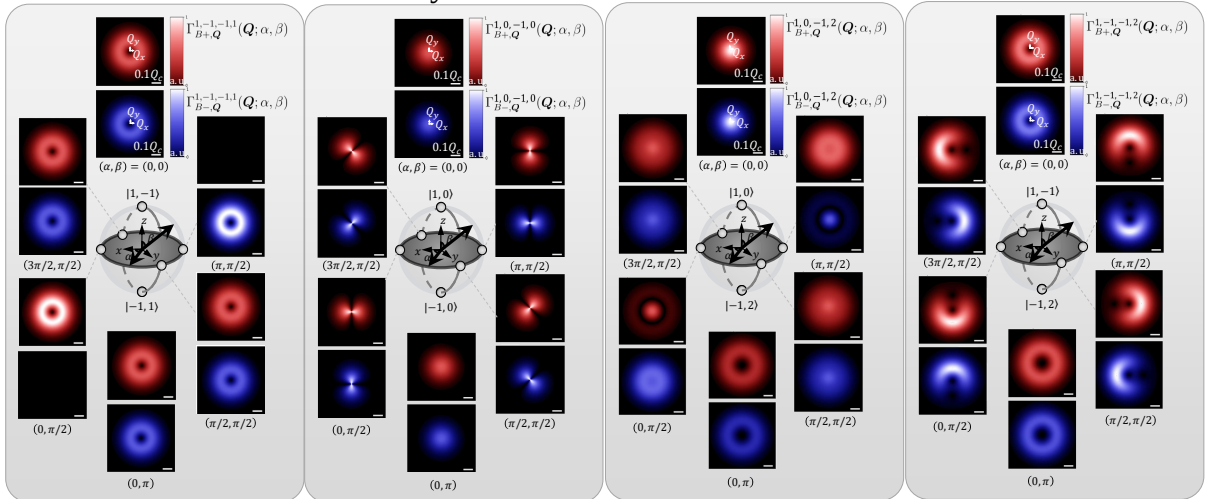
Valley-mixed excitons transition rate
