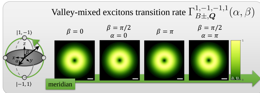
Figure 3.3 : Normalized transition rate of total BXs excited by the VVB state |1, -1, -1, 1; \alpha, \beta\rangle in momentum space.
