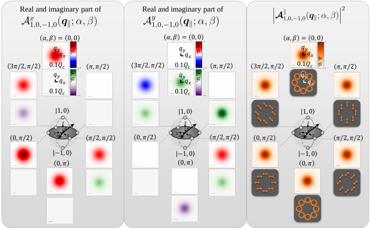
Figure 2.8 : Real and imaginary parts of \mathcal{A}_{1,0,-1,0}^x(\mathbf{q}_{\parallel}; \alpha, \beta) and \mathcal{A}_{1,0,-1,0}^y(\mathbf{q}_{\parallel}; \alpha, \beta) , together with the squared magnitude and polarization distribution of \mathcal{A}_{1,0,-1,0}^{\parallel}(\mathbf{q}_{\parallel}; \alpha, \beta) .
