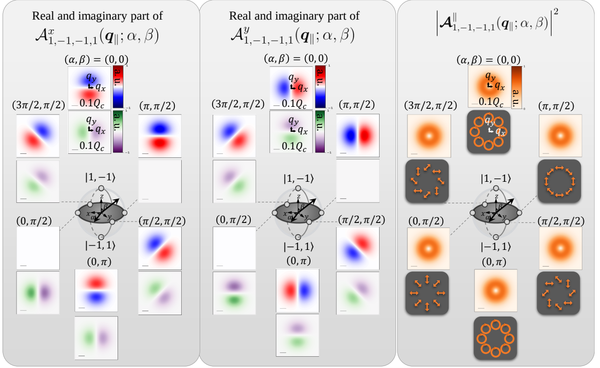
Figure 2.9 : Real and imaginary parts of \mathcal{A}_{1,-1,-1,1}^x(\mathbf{q}_{\parallel}; \alpha, \beta) and \mathcal{A}_{1,-1,-1,1}^y(\mathbf{q}_{\parallel}; \alpha, \beta) , together with the squared magnitude and polarization distribution of \mathcal{A}_{1,-1,-1,1}^{\parallel}(\mathbf{q}_{\parallel}; \alpha, \beta) .
