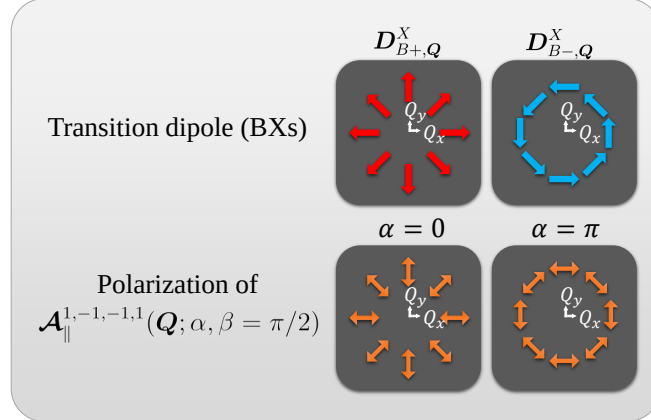
Figure 3.1 : Illustration of the transition dipole moments of valley-mixed BXs [6], and their matching with the transverse polarization of the VVB states |1, -1, -1, 1; \alpha = 0, \beta = \pi/2\rangle and |1, -1, -1, 1; \alpha = \pi, \beta = \pi/2\rangle in momentum space.
