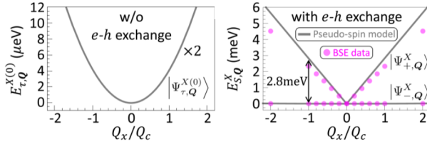
Figure 1.4 : The lowest valley-degenerate (left) and valley-split (right) exciton bands in MoS 2 along the Q_x direction, reproduced from Ref. [6].
